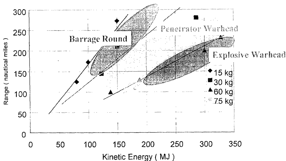
FIGURE 8. The projectile range for varied mass and the initial projectile kinetic energy.
