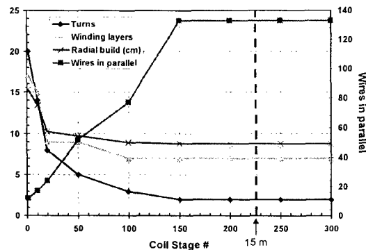
Figure 4. Variation of coil parameters from the breech to muzzle of a 15 or 20 m gun for SLINGSHOT simulation assuming PBO/carbon fiber/epoxy reinforcement shells. All coils have the same winding length of 49 mm at 58 mm center-to-center spacing.
