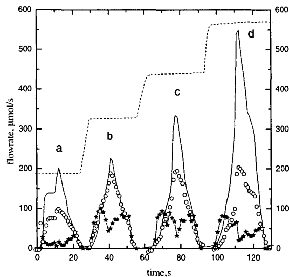
Fig. 5 : Time course of NO flow rate through the 2 nd injector (.....) and HI flow rate through the 3 rd injector (—), rate of formation of atomic iodine detected by ISD in the cell 11 (—*—) and visible photometry in the cell 12 (○), respectively. Total pressure 2.1 kPa, 220 \mu\text{mol ClO}_2/\text{s} and 2 mmol \text{N}_2/\text{s} in the primary flow, d_{1-2} = 38 \text{ mm} , d_{2-3} = 3.7 \text{ mm} , d_{3-\text{ISD}} = 10 \text{ mm} .
