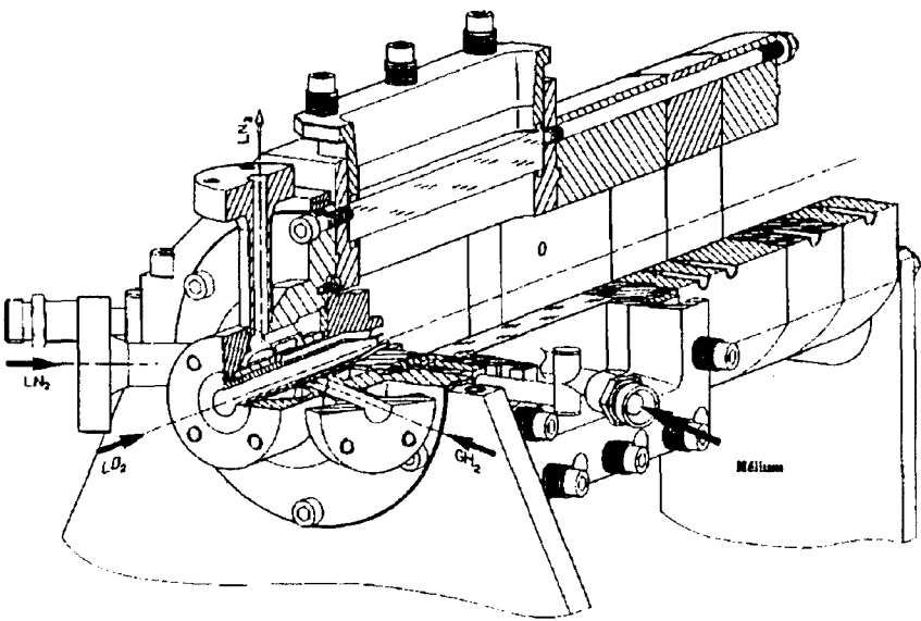
Figure 1: Mascotte Combustor
