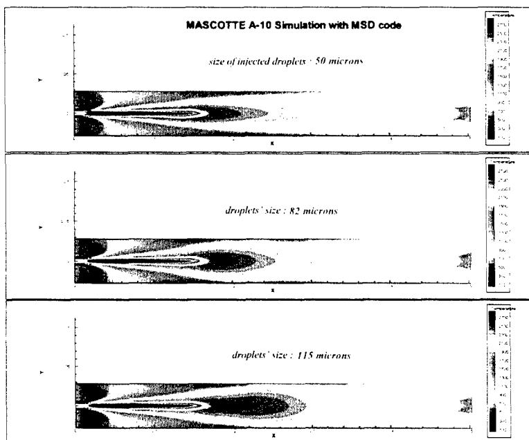
Figure 7 : Temperature field - Effect of droplet size diameter
