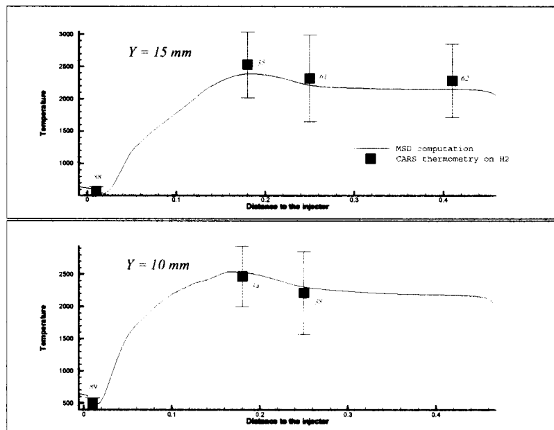
Figure 14 : Temperature axial profiles - Comparison of computations and experimental data ( y = 10 mm and y = 15 mm)
