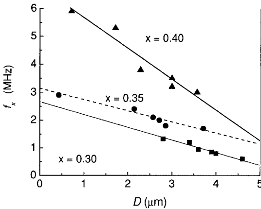
Figure 2. Linear relationship between relaxation frequency and grain size for the studied compositions.
