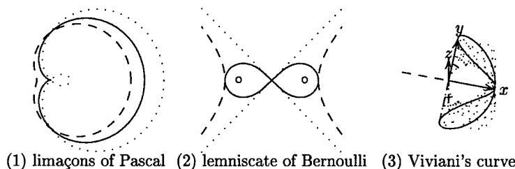
Fig. 4. Rational quartics on Dupin cyclides.
