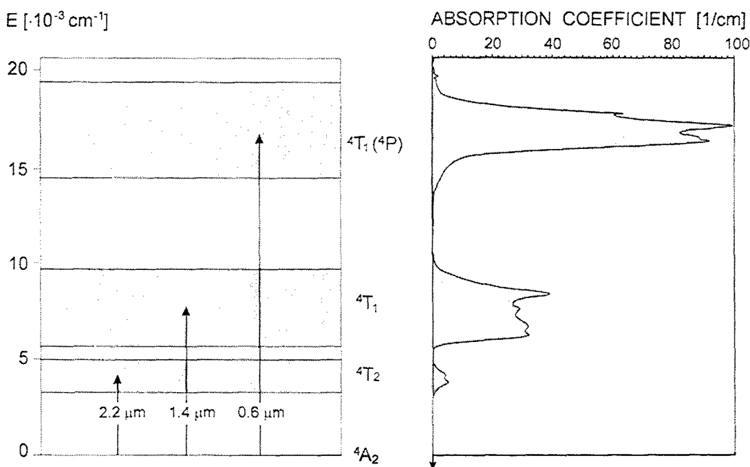
Fig. 2. Energy levels for \text{Co}^{2+} in tetrahedral sites and room temperature \text{YAG}:\text{Co}^{2+} (2 at.% \text{Co}^{2+} ) absorption spectra
