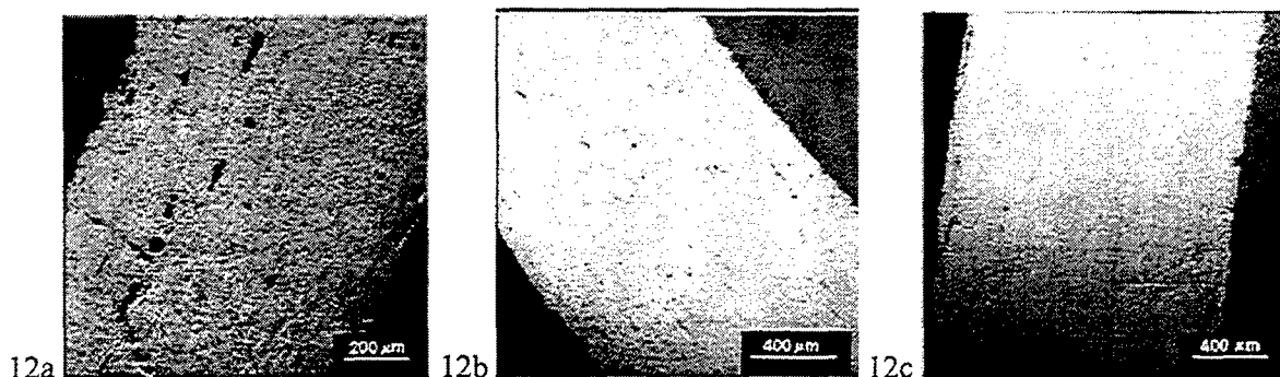
Figure 12. SEM micrographs of as-sprayed (a) \text{HfB}_2 , (b) \text{HfC} and (c) \text{HfN} .
