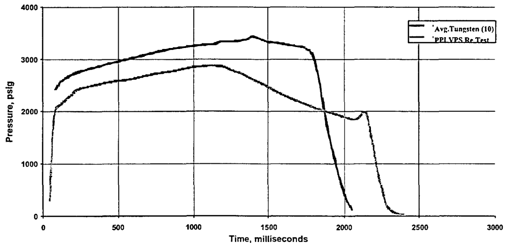
Figure 8: Pressure trace data for the VPS Re 5 inch CP test
