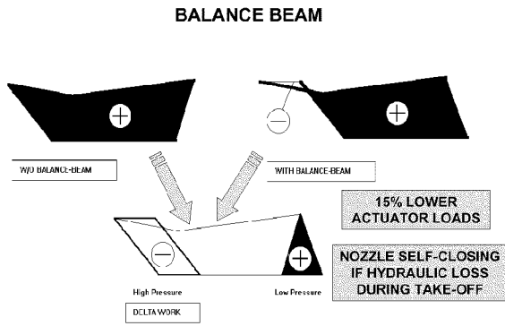
Fig. 15.- Balance Beam effect
