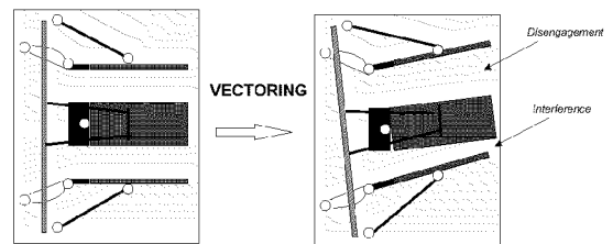
Fig. 14a.- Vectoring with simple reaction bars
