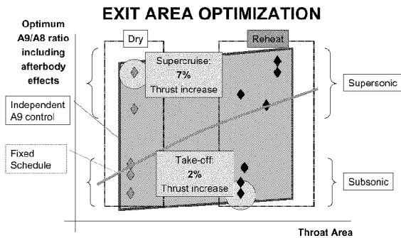
Fig. 4.- Optimization of Nozzle Exit Area
