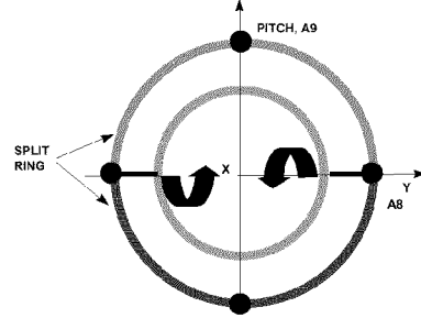
Fig. 13.- "Two-Ring" Pitch-only Nozzle
