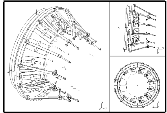
Fig. 9.- Nozzle Movement in vectoring
