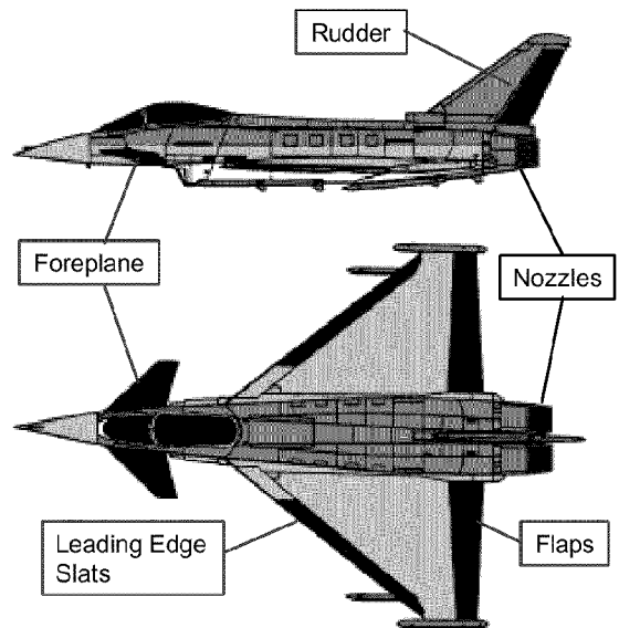
Fig. 5.- Redundant Flight Controls with TVNs
