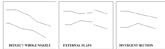
Fig. 6.- Existing types of 3-D TVNs
