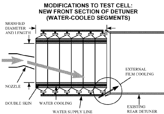
Fig. 17.- Modifications to Test Cell
