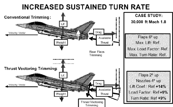
Fig. 3.- Increased Sustained Turn Rate with TVNs
