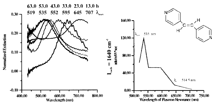
Figure 2. Extinction spectra and height-scanned excitation profile for trans -alkene stretch of BPE of Ag PPA surface.
