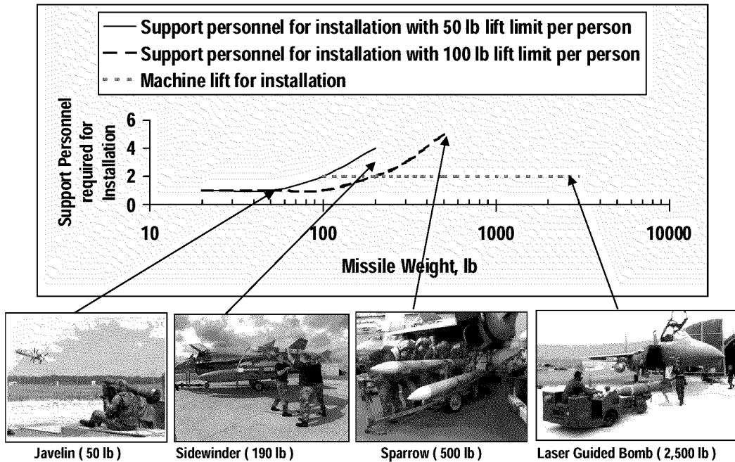
Figure 9. Logistics Is Simpler for Light Weight Missiles.
