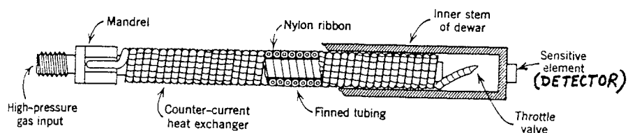
(a) Construction of a Cryostat
