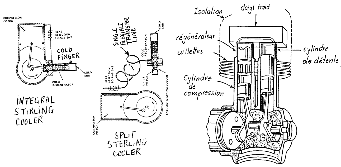
Fig.10. Views of the integral-Stirling cycle cooler (left) and the more recent split-Stirling cycle cooler (right). The latter allows the compressor to be conveniently located [Photonics Spectra, Oct 89, p.76]
