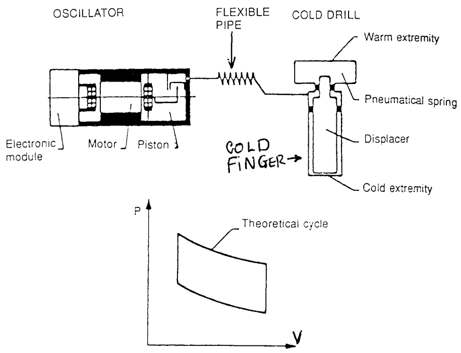
Fig.A11. Split Stirling cooler and Stirling heating cycle.
