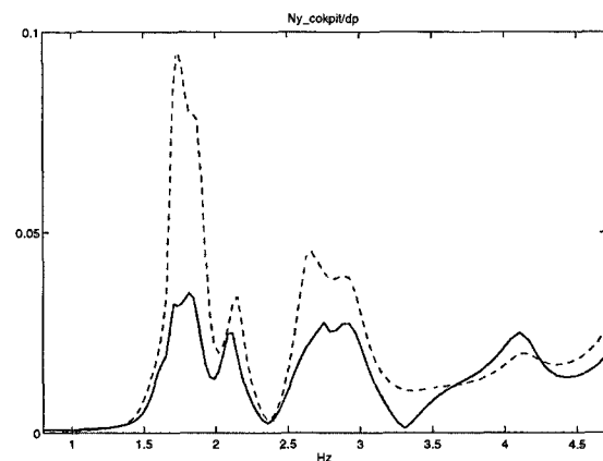
Figure 13: Minimization of pilot coupling transfer:
