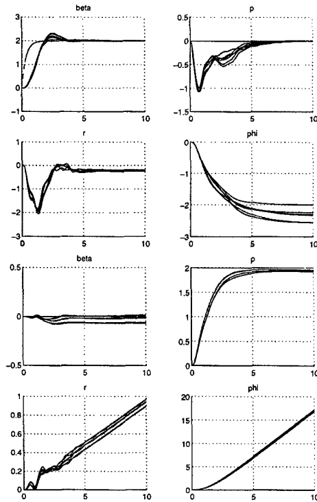
Figure 11: Illustration of robust performance for pilot demand in the time domain
