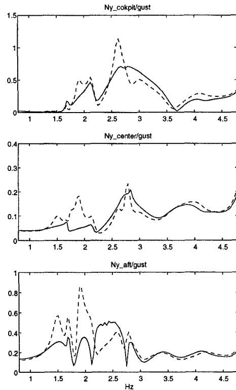
Figure 12: Illustration of gust alleviation performance in the frequency domain
