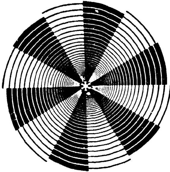
MAW Spiral Antenna 1.5 Turns/Octave
