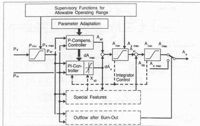
Pressure Controller Block Diagram
