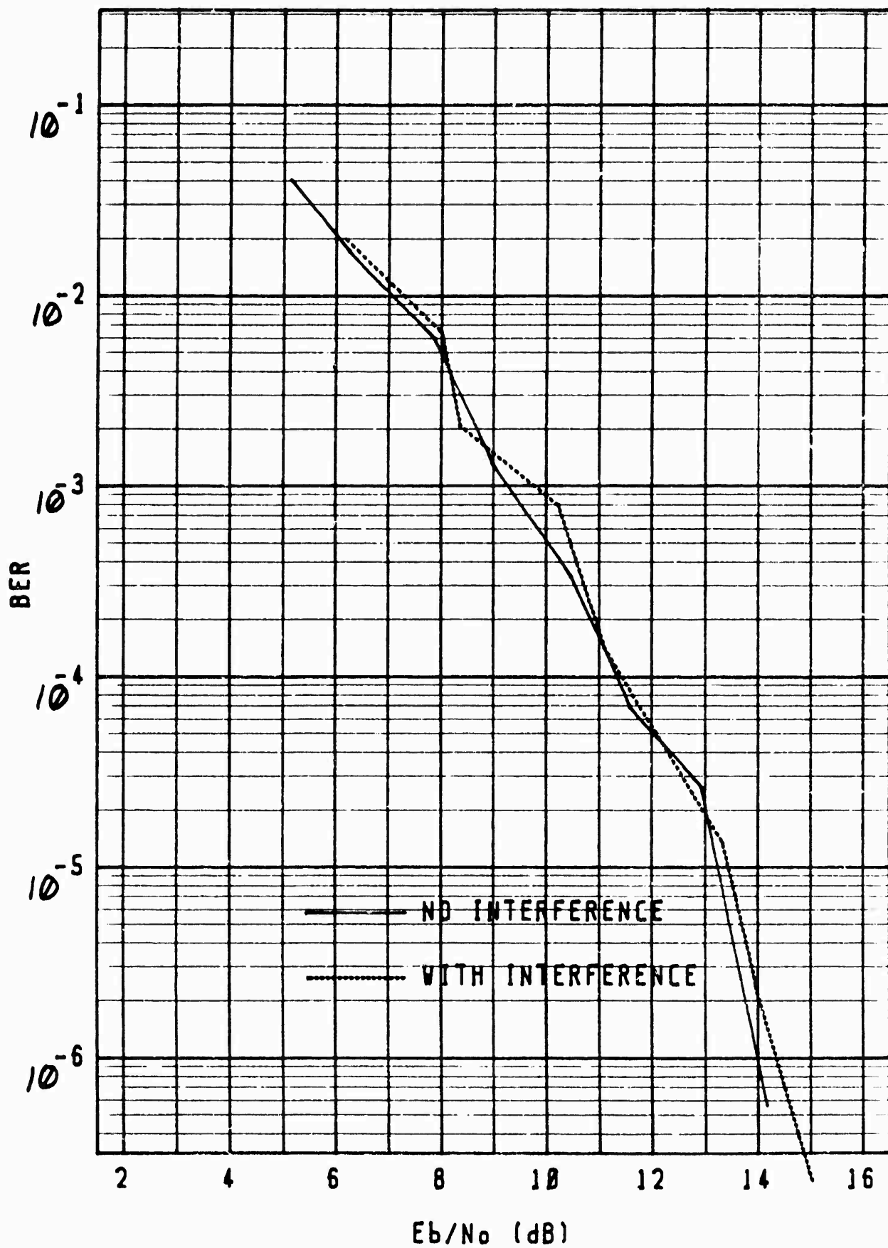
Figure 14 Bit-Error-Rate During Interference Test
