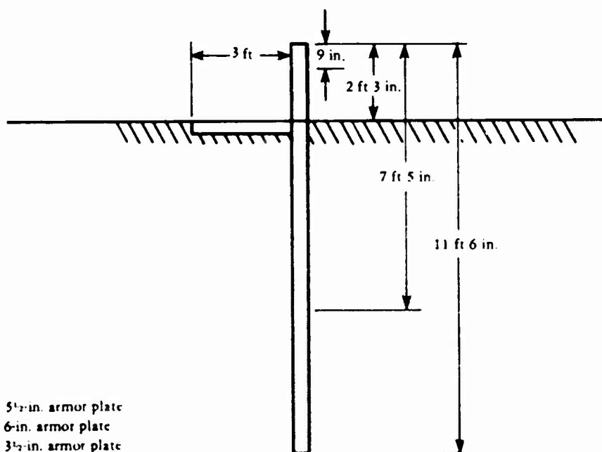
Figure 3. Test wall.
