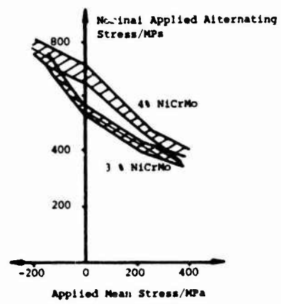
Figure 6 Goodman Diagram (RM Diagram) Showing Endurance Limits for 4% NiCrMo and 3 1/2% NiCrMo Steel
