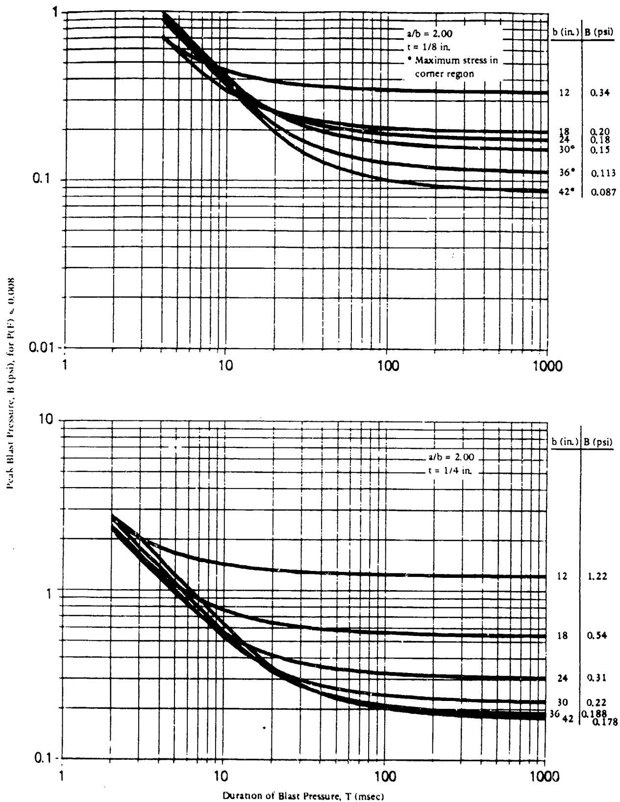
Figure 16. Peak blast pressure capacity for annealed glass panes: a/b = 2.00 , \tau = 1/8 and 1/4 in.
