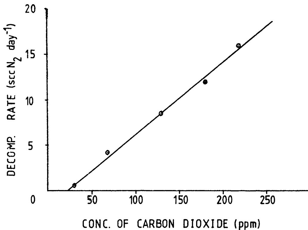
FIGURE 1. PLOT OF HYDRAZINE DECOMPOSITION RATE IN A 304L VESSEL AT 60°C AGAINST TOTAL CONC. OF DISSOLVED CARBON DIOXIDE
