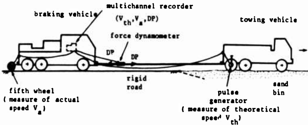
Fig.9 Traction test.
