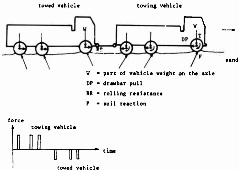
Fig. 1 Forces acting on the soil during compaction.
