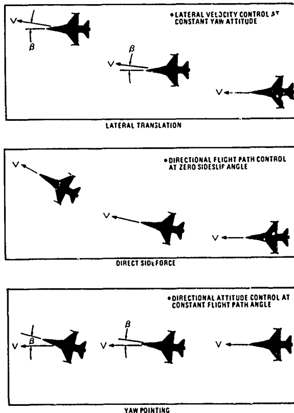
Figure 9 Lat-Dir Decoupled Options
