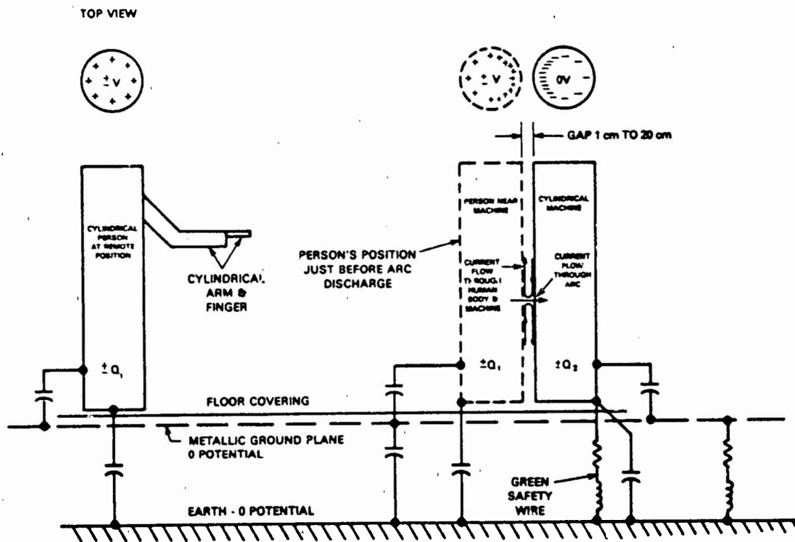
Fig. 1 - Electrostatic buildup and discharge model
