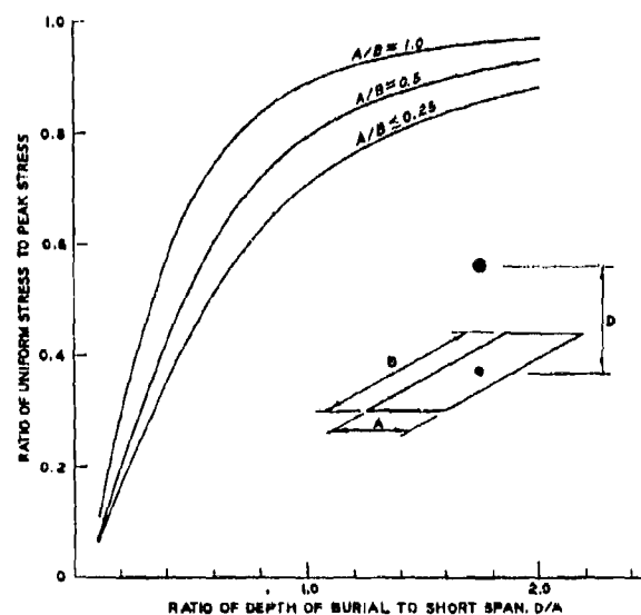
Figure 4. Equivalent uniform load in flexure
