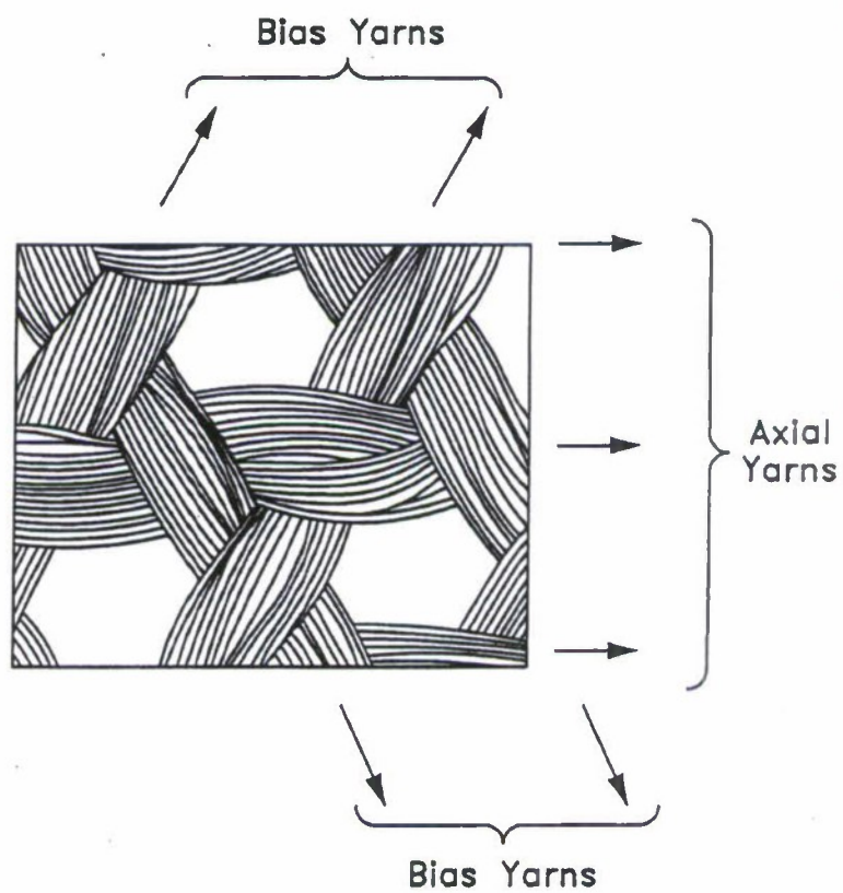
FIG. 18 (PRIOR ART)
