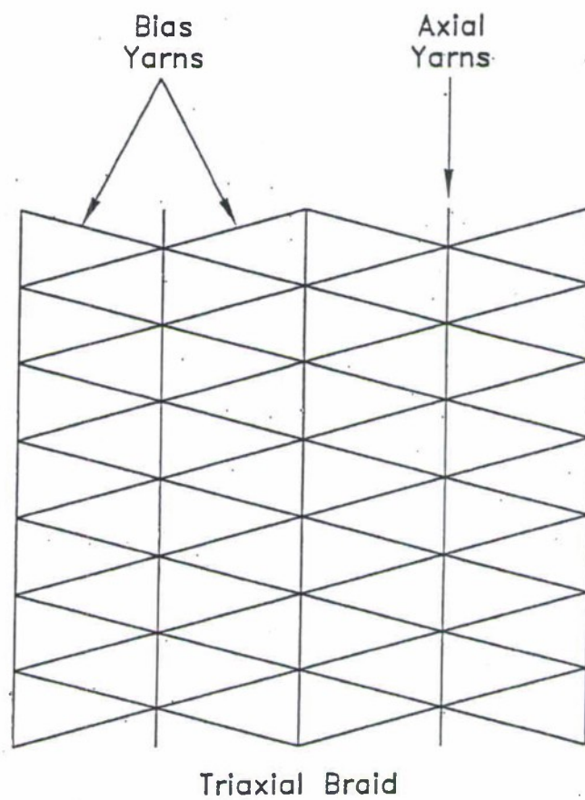
FIG. 13 (PRIOR ART)
