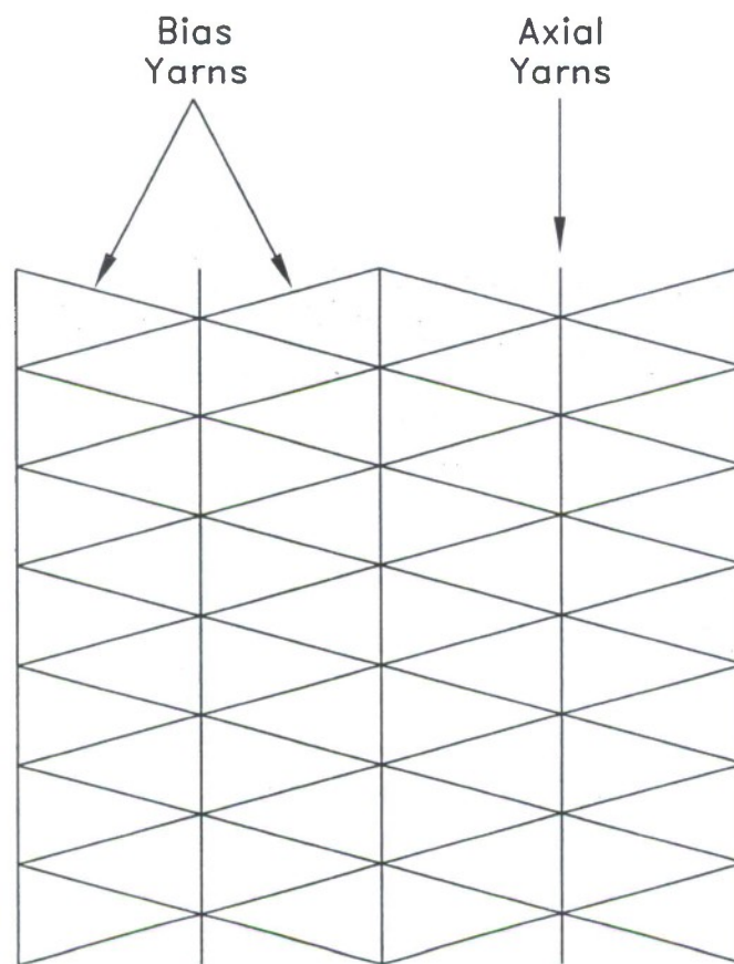
Triaxial Braid
