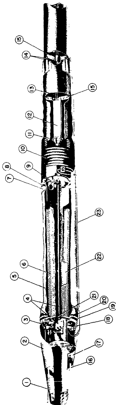
Fig. 12 THE 3F6 COBRA, LATEST MODEL OF THE 6-INCH UNIT USED FOR COMBUSTION RESEARCH, COM-BUSTOR DEVELOPMENT AND ALLIED STUDIES.
