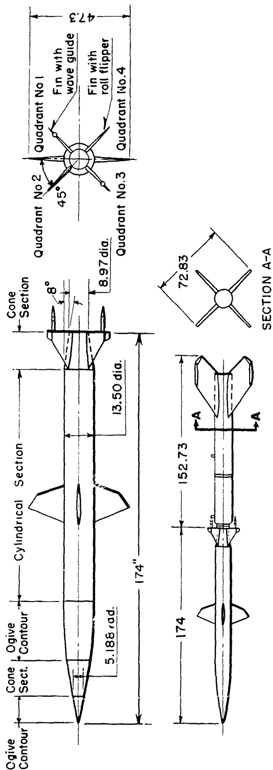
Fig. 13 AERODYNAMIC CONFIGURATION OF TERRIER.
