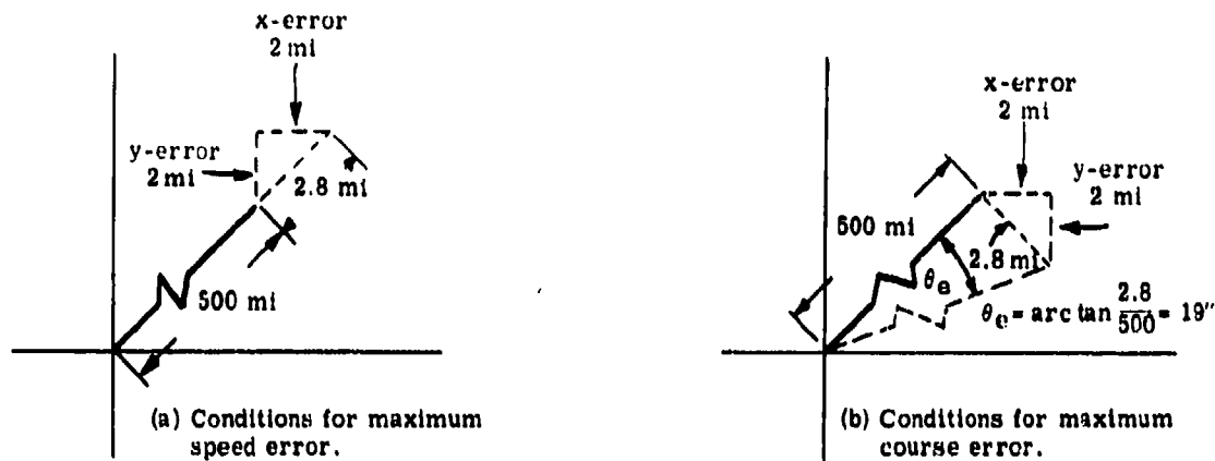
Figure 10 - Determination of speed and coarse errors
