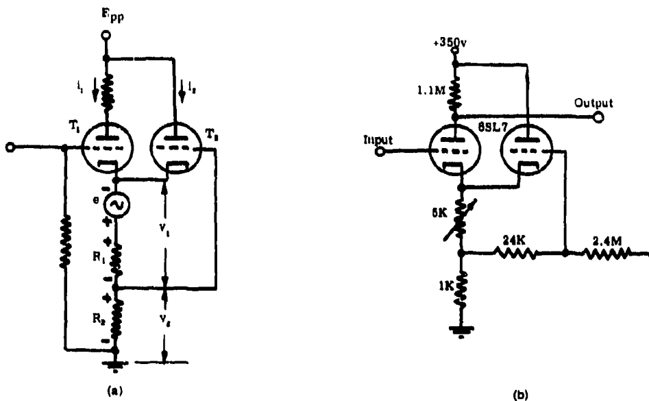
Figure 9 - Circuit for compensating for the effects of heater voltage change
