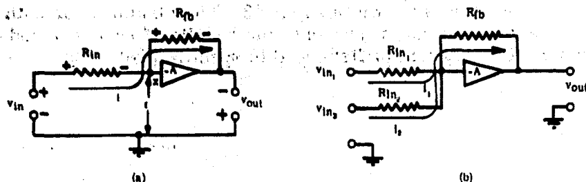
Figure 5 - Sign-changing and summing amplifiers
