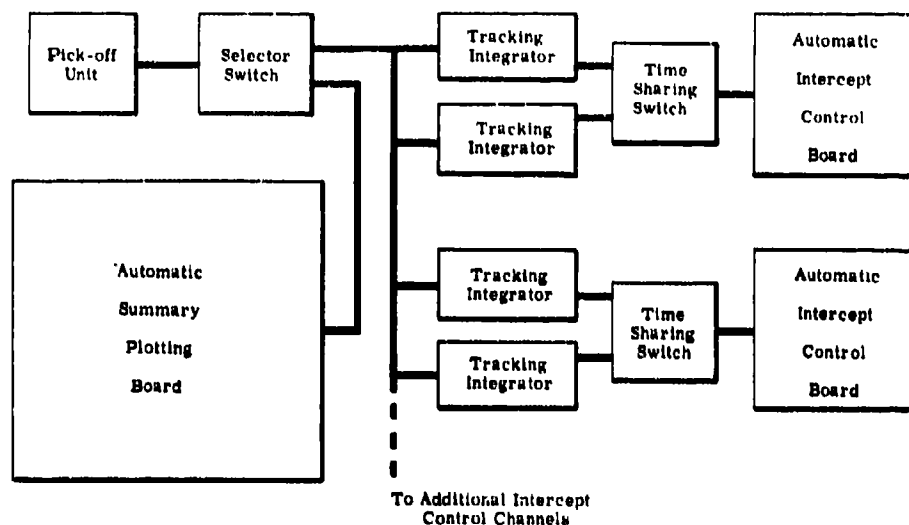
Figure 1 - Block diagram of interim intercept control system
