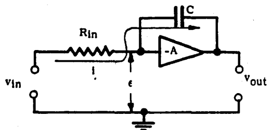
Figure 6 - Integrating amplifier
