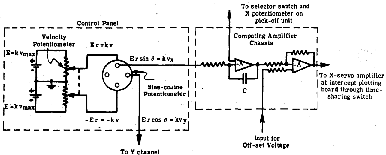
Figure 4 - Simplified tracking integrator schematic
