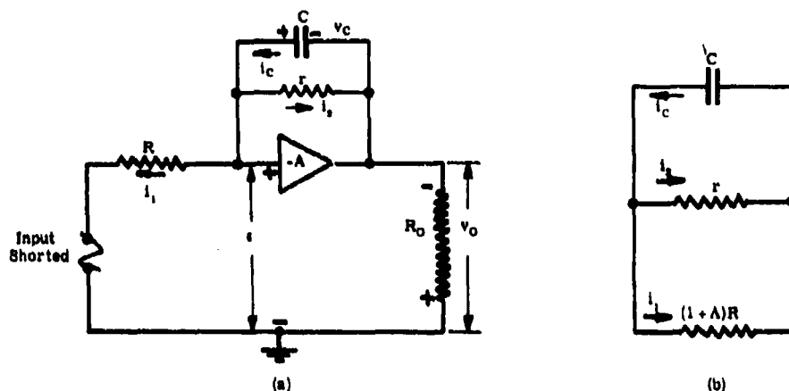
Figure 11 - Discharge paths in the integrating amplifier
