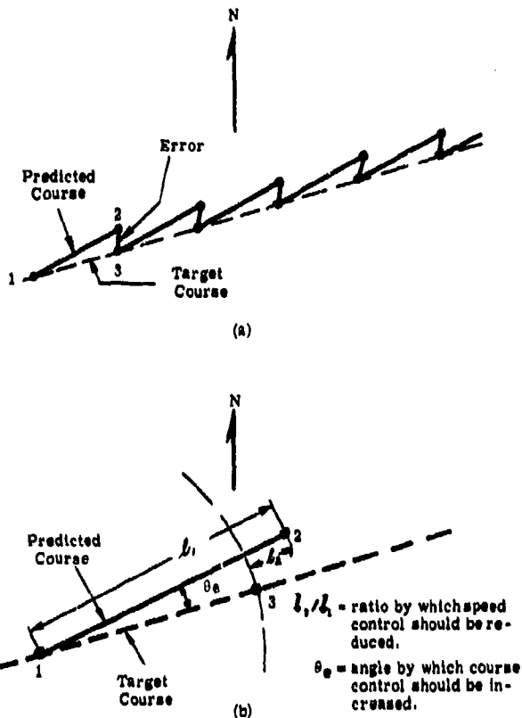
Figure 7 - Plotted tracks with course and speed errors
