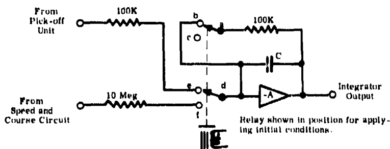
Figure 12 - Method of applying initial conditions
