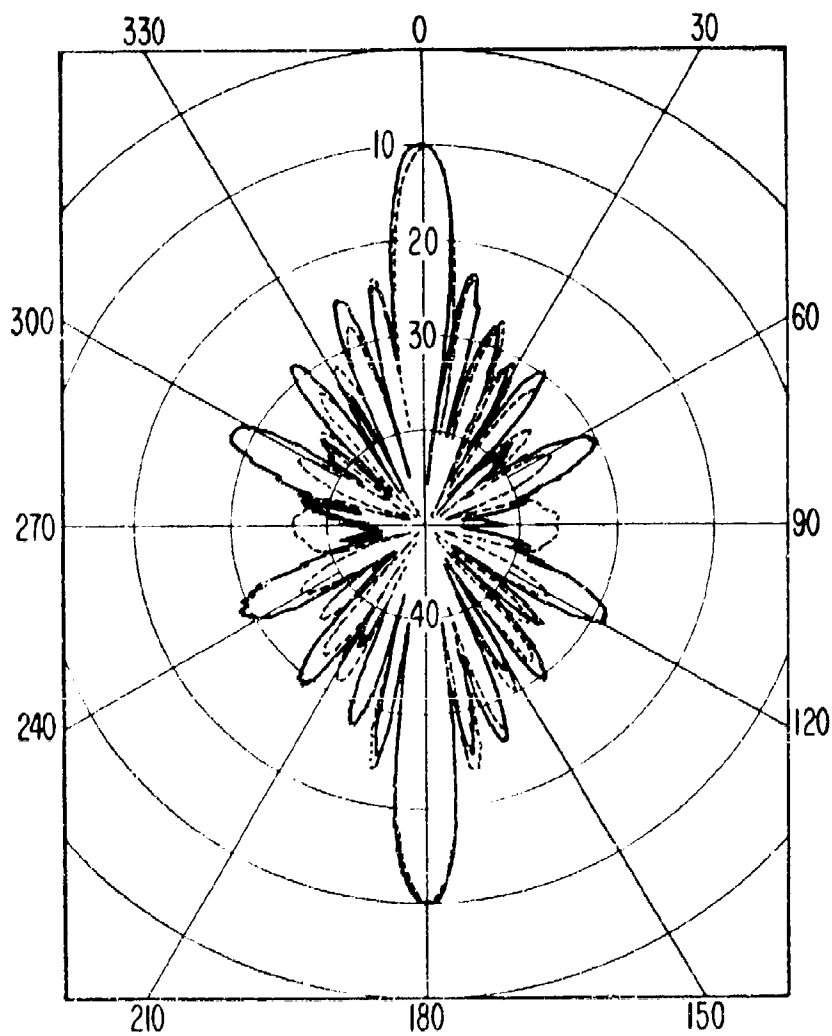
(U) Fig. B1 — 18-ft line array directivity pattern at 2 kHz by nearfield technique and computed farfield
