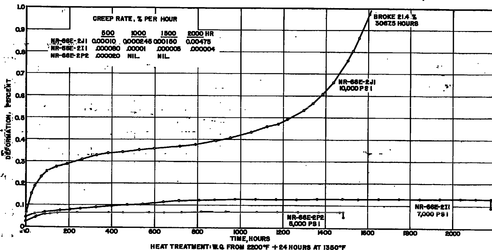
FIGURE 25—TIME-DEFORMATION CURVES AT 1500°F FOR LOW-CARBON N-155 ALLOY DISC, NR-66E-2R.
