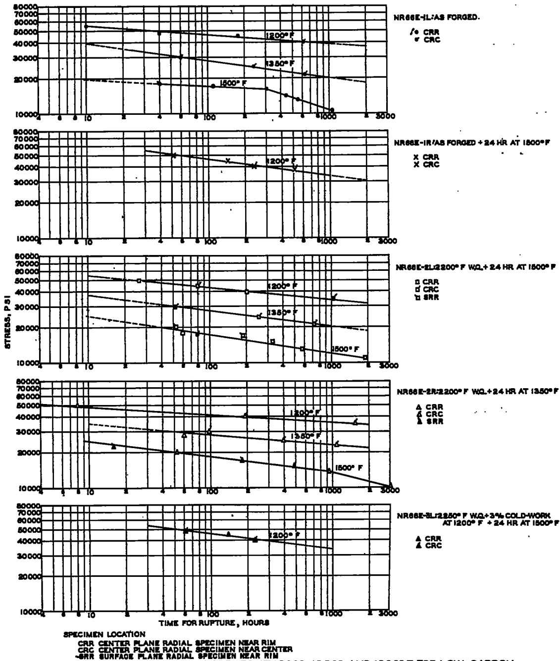
FIGURE 6.—STRESS-RUPTURE-TIME CURVES AT 1200°, 1350°, AND 1500° F FOR LOW-CARBON N155 ALLOY DISCS, NR66E.
