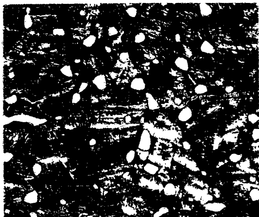
Figure 22. Heat H245, 3.5% Ni. Quenched from 1550°F. in the alpha + beta field. Islands of alpha (light) appear in an acicular alpha (transformed beta) matrix.
