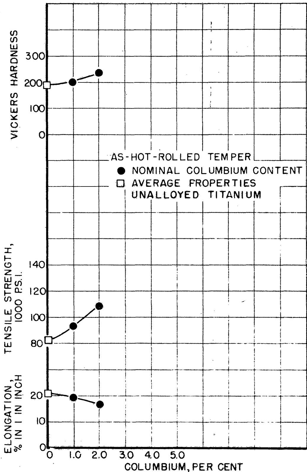
FIGURE 30. EFFECT OF COLUMBIUM ON THE PROPERTIES OF AS-HOT-ROLLED PROCESS A TITANIUM SHEET
