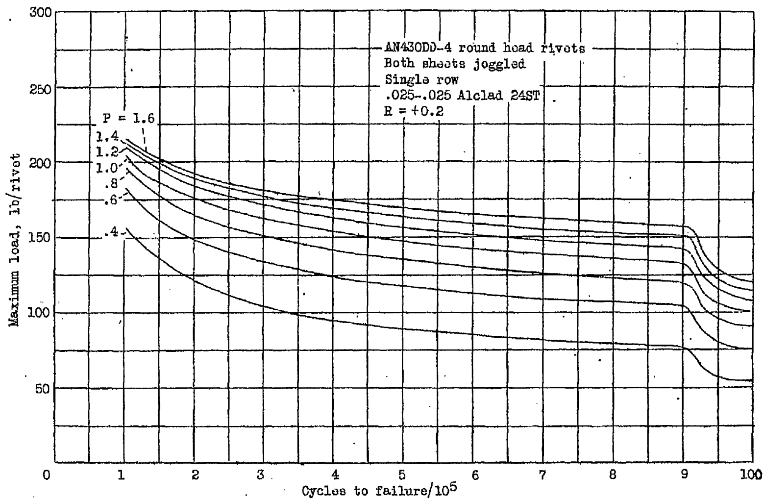
Figure 21.- Effect of rivet pitch upon fatigue strength, interpolated curves.
