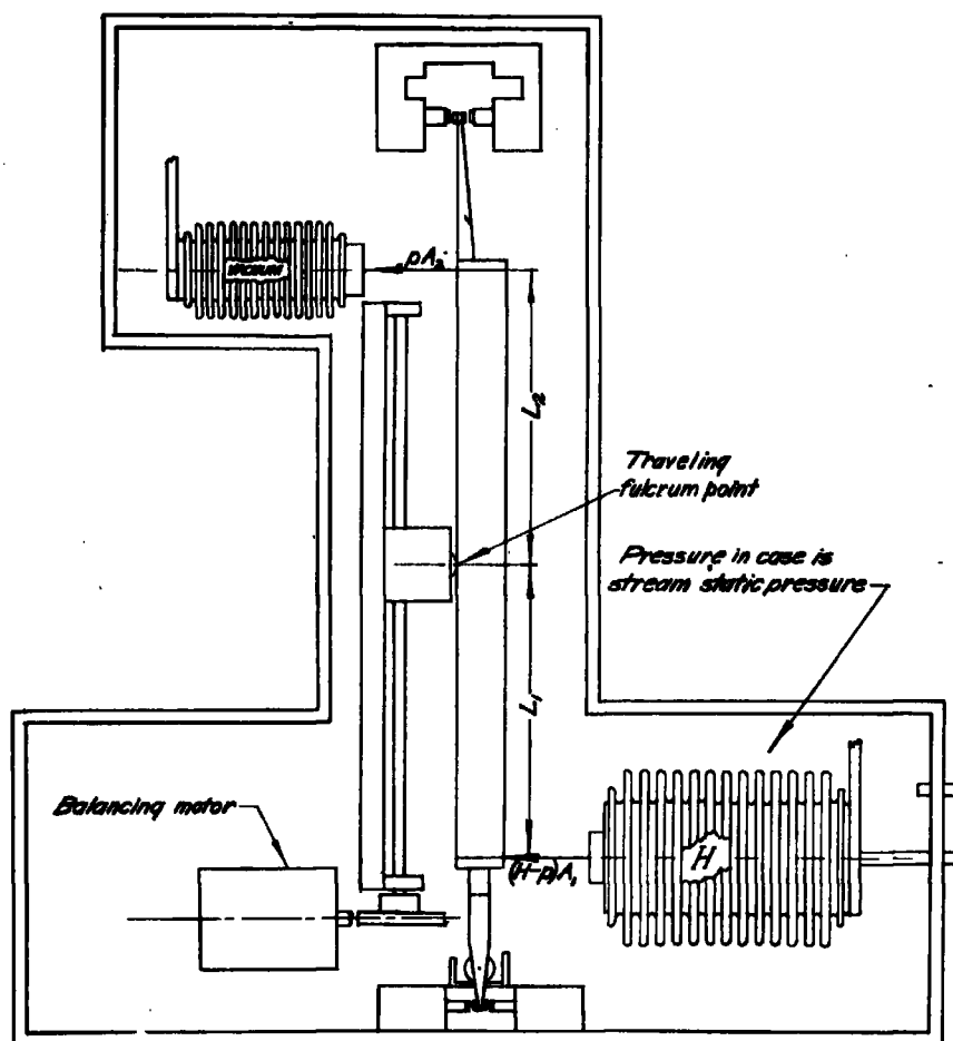
Figure 3-Schematic diagram showing forces at balance.
