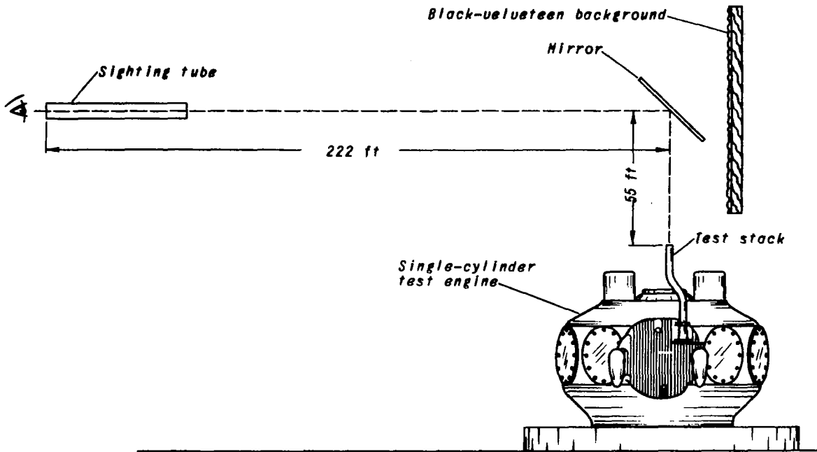
Figure 3. - Visibility-test setup.
