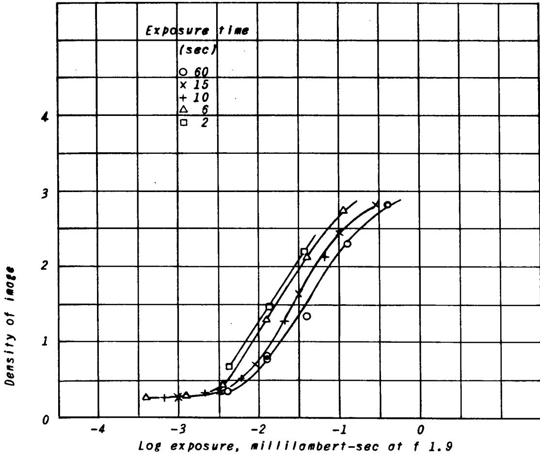
Figure 2. - Sample densitometric curves for Tri-X Aero Safety film.
