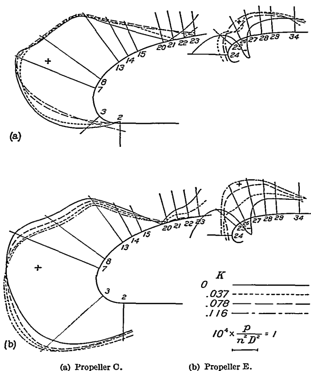
FIGURE 11.—Pressure distribution on nose 1, slot 2. Opening 4\frac{1}{2} in.; 1/\sqrt{P_c}=0 .
