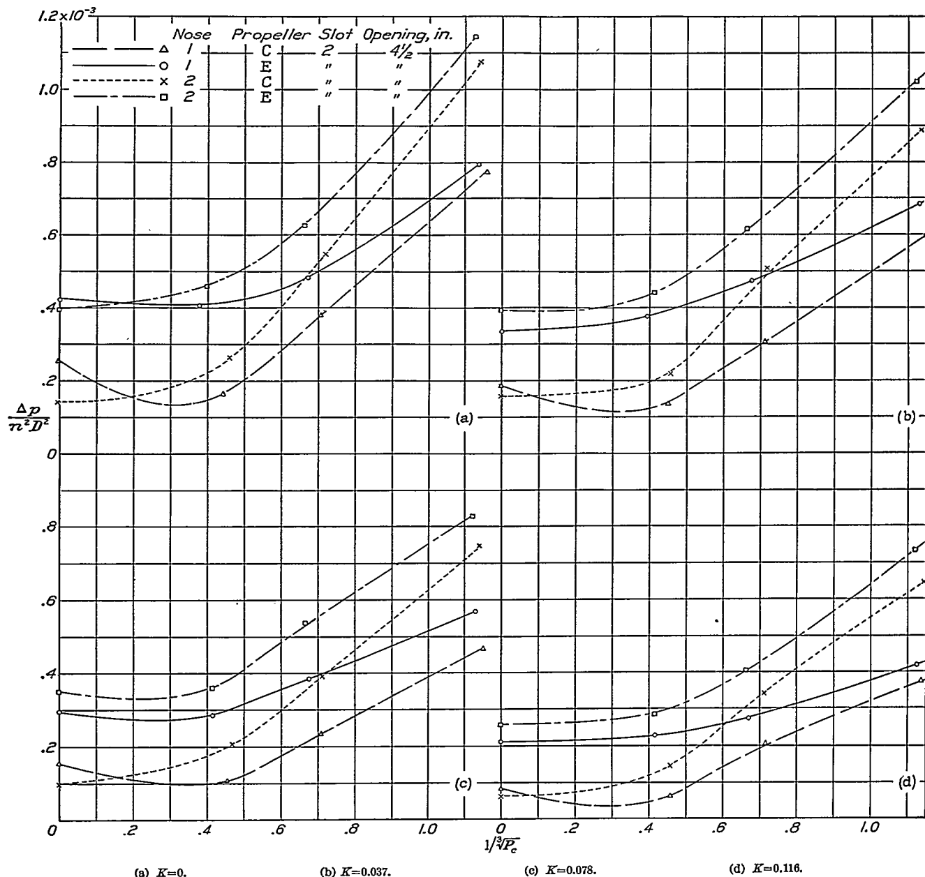
FIGURE 4.—Curves of \frac{\Delta p}{n^2 D^2} against 1/\sqrt{P_c} for one slot on each nose for propellers C and E set 20^\circ at 0.75R .
