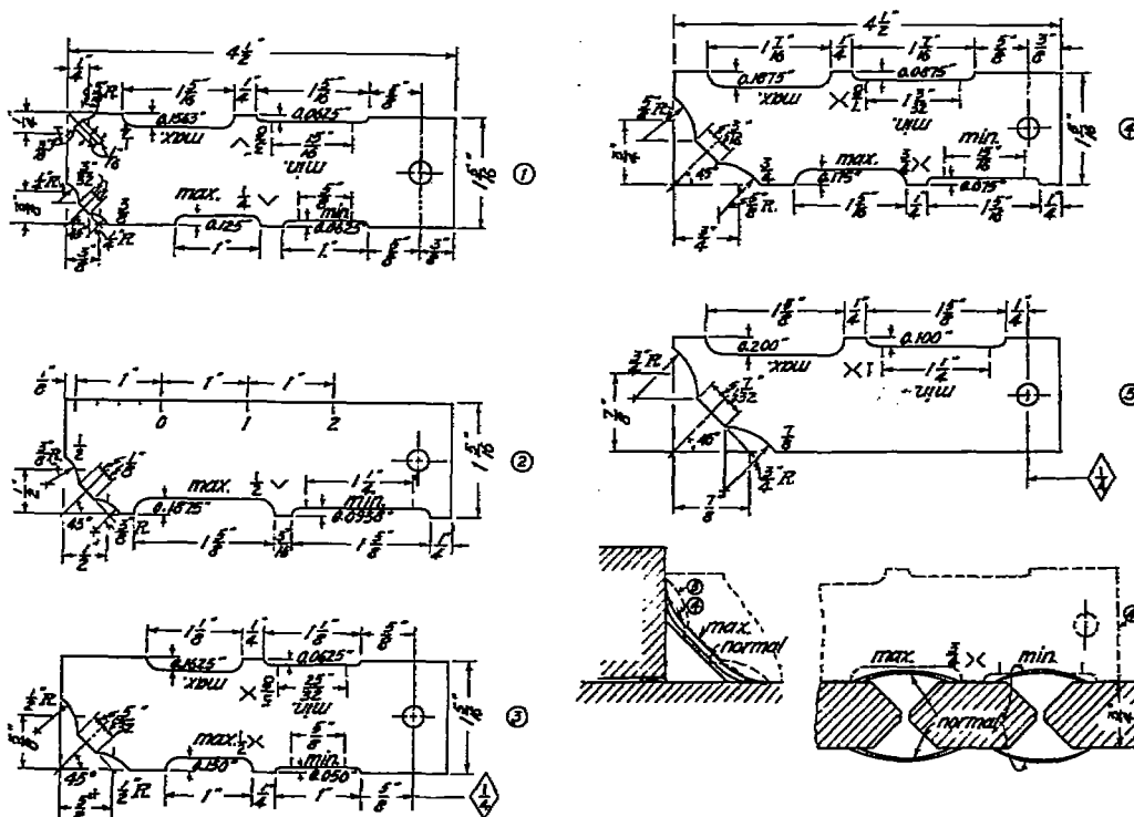
FIGURE M.—Gages for measuring butt and fillet welds and a sketch illustrating method of application of these gages
