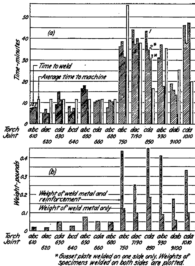
FIGURE 31.—Time required to machine and weld joints; weights of weld metal and reinforcement
