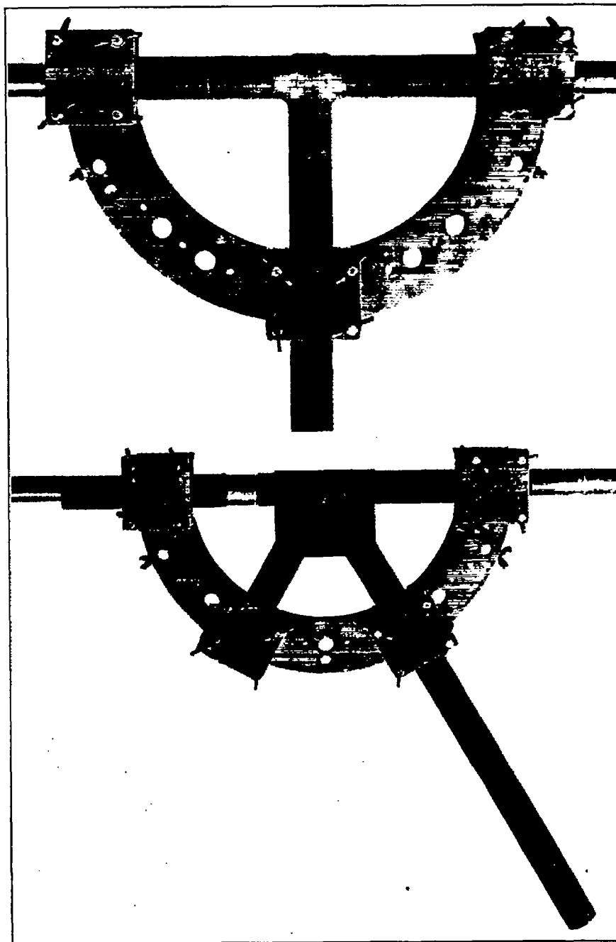
FIGURE 18.—A T joint (upper) and a lattice joint (lower) set up in the jig for welding. The tubes are clamped in V blocks bolted to the frame. Where tubes of different diameter were welded together, shims were placed under the blocks holding the small tubes. The jig may be turned over for welding on the bottom side.
