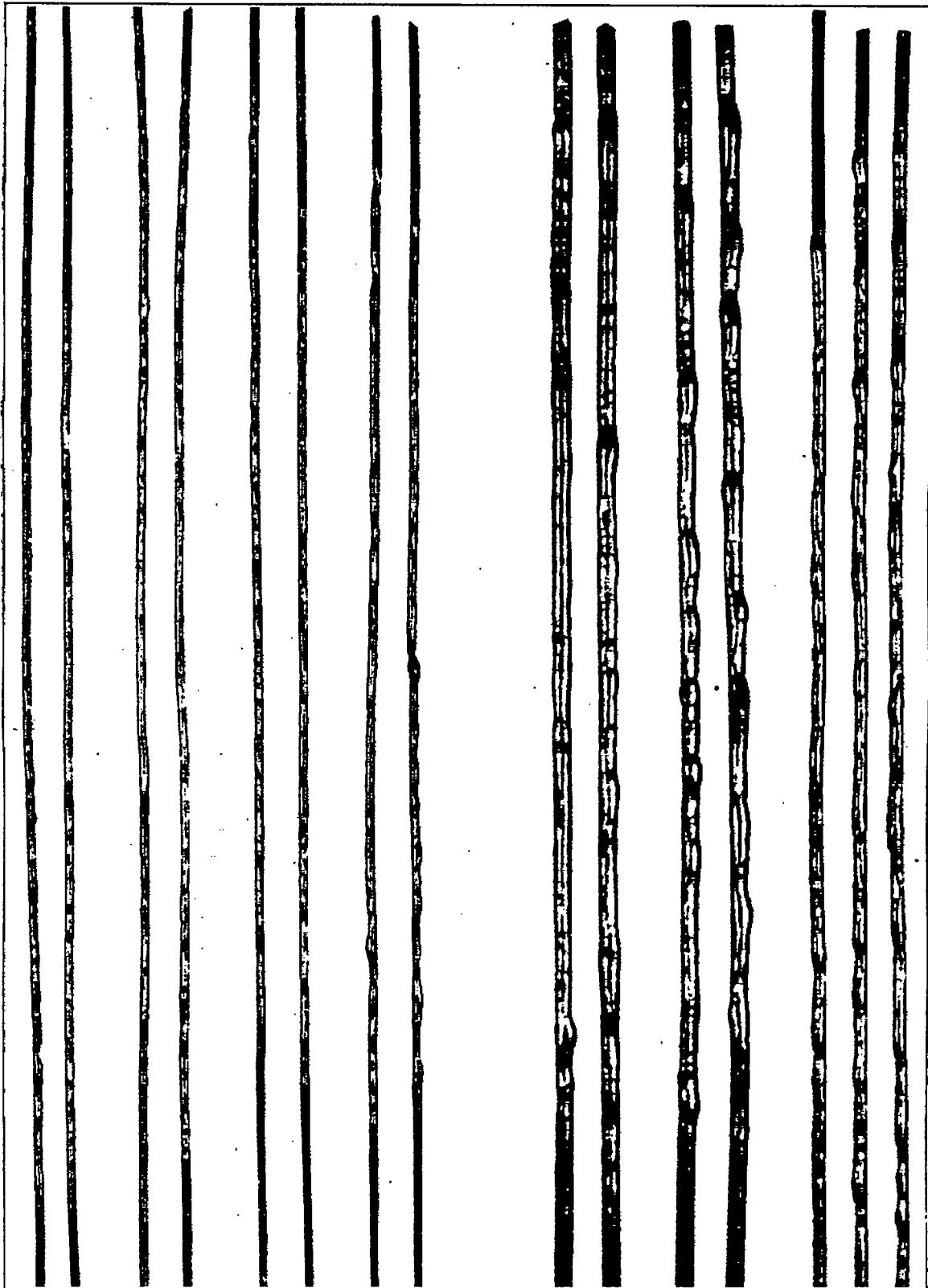
FIGURE 4.—Welding wire after the flame test. The samples were melted with the torch and their behavior observed in the same manner as for the base metal
