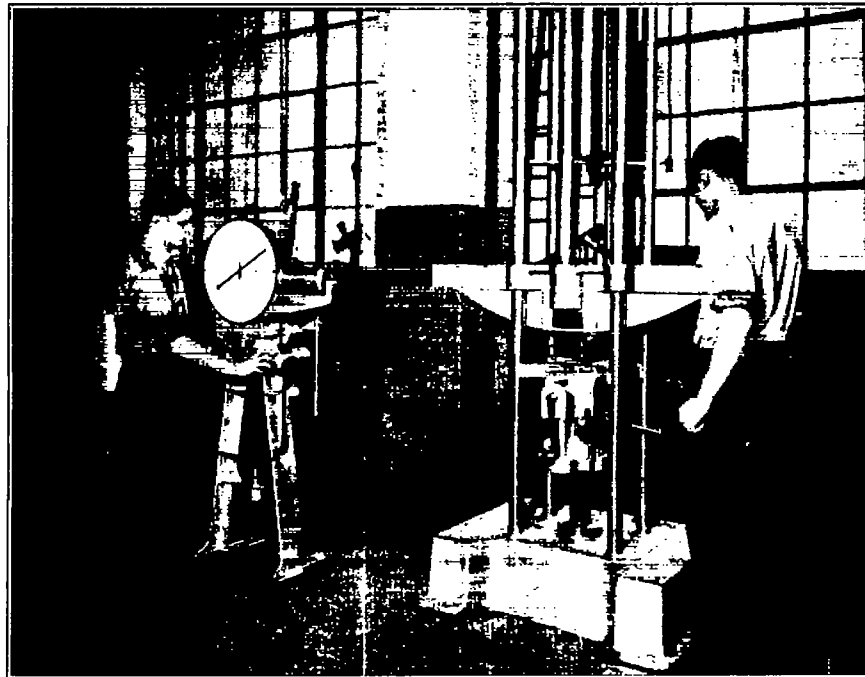
FIGURE 9.—A lattice joint being tested
