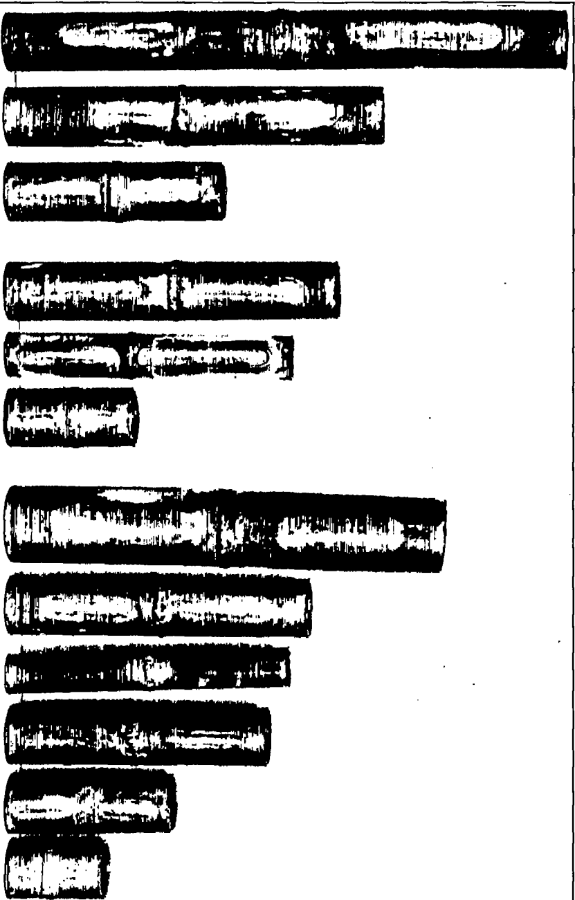
FIGURE 5.—Butt joints made to determine the weldability of the rod
