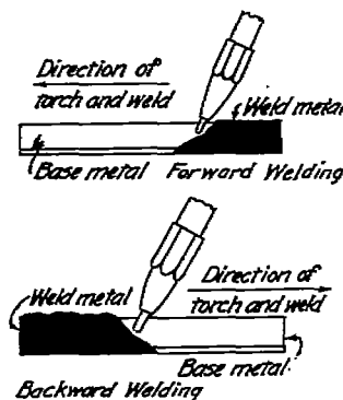
FIGURE L.—Methods of welding
