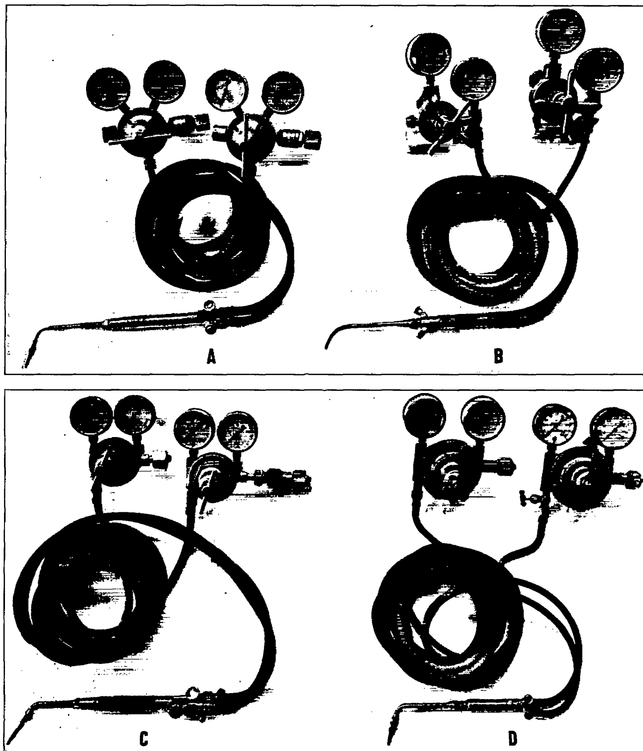
FIGURE 11.—The torches and equipment used to weld the specimens. Each torch was used to weld about an equal number of specimens.
