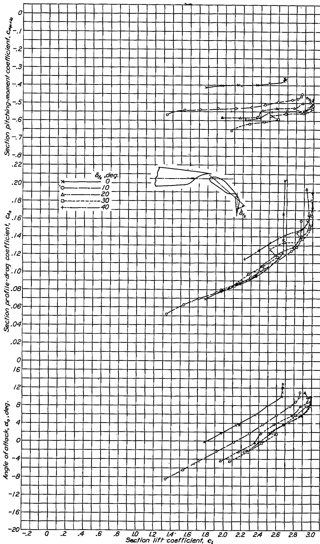
FIGURE 24—Section characteristics of the N. A. O. A. 23012 airfoil with the main slotted flap deflected 40° and the auxiliary 0.10c s slotted flap deflected various amounts.
