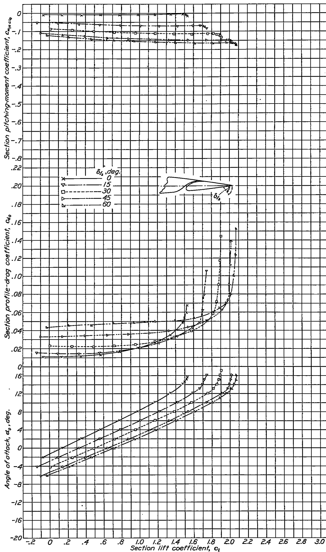
FIGURE 4.—Section characteristics of the N. A. C. A. 23012 airfoil with the main slotted flap deflected 0^\circ and the auxiliary 0.05c_w split flap deflected various amounts.
