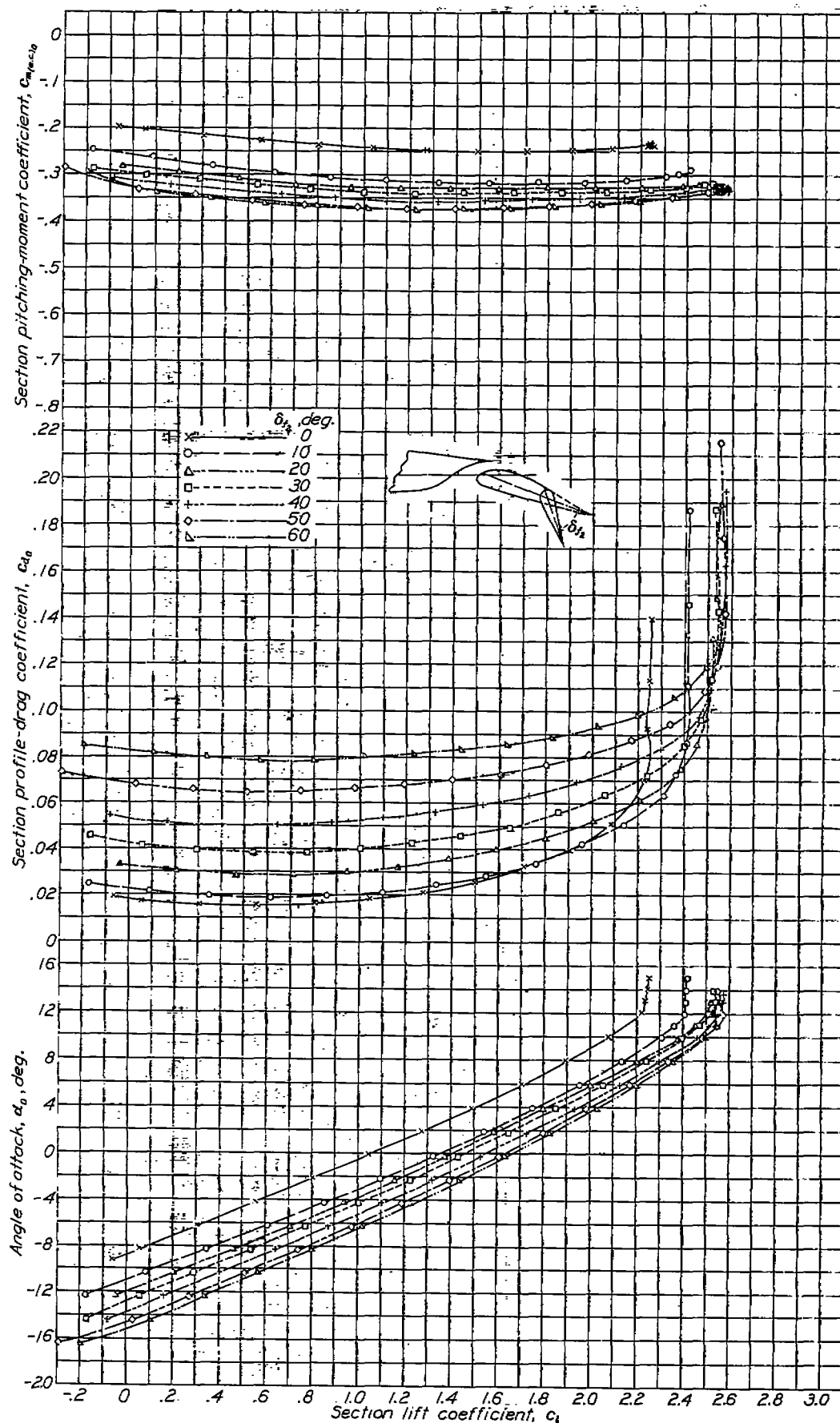
FIGURE 18.—Section characteristics of the N. A. C. A. 23012 airfoil with the main slotted flap deflected 20° and the auxiliary 0.10c w plain flap deflected various amounts.
