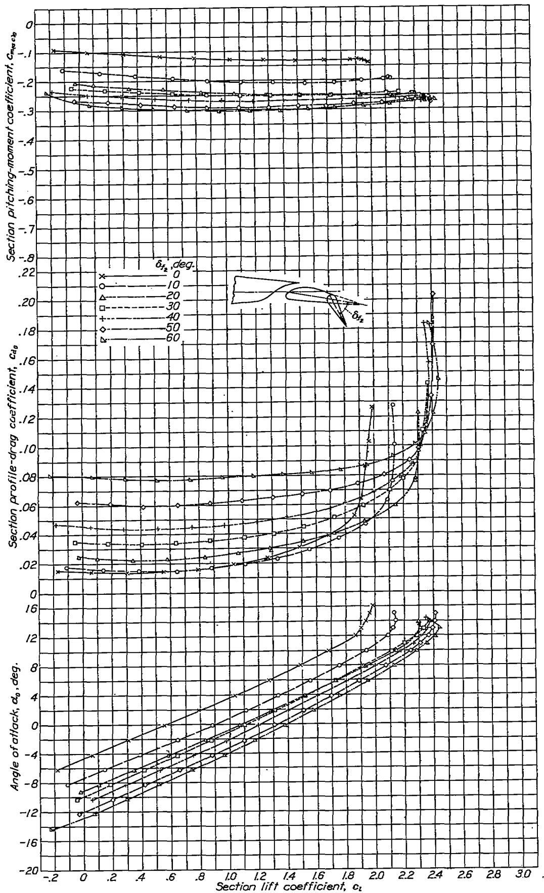
FIGURE 17.—Section characteristics of the N. A. C. A. 23012 airfoil with the main slotted flap deflected 10^\circ and the auxiliary 0.10c plain flap deflected various amounts
