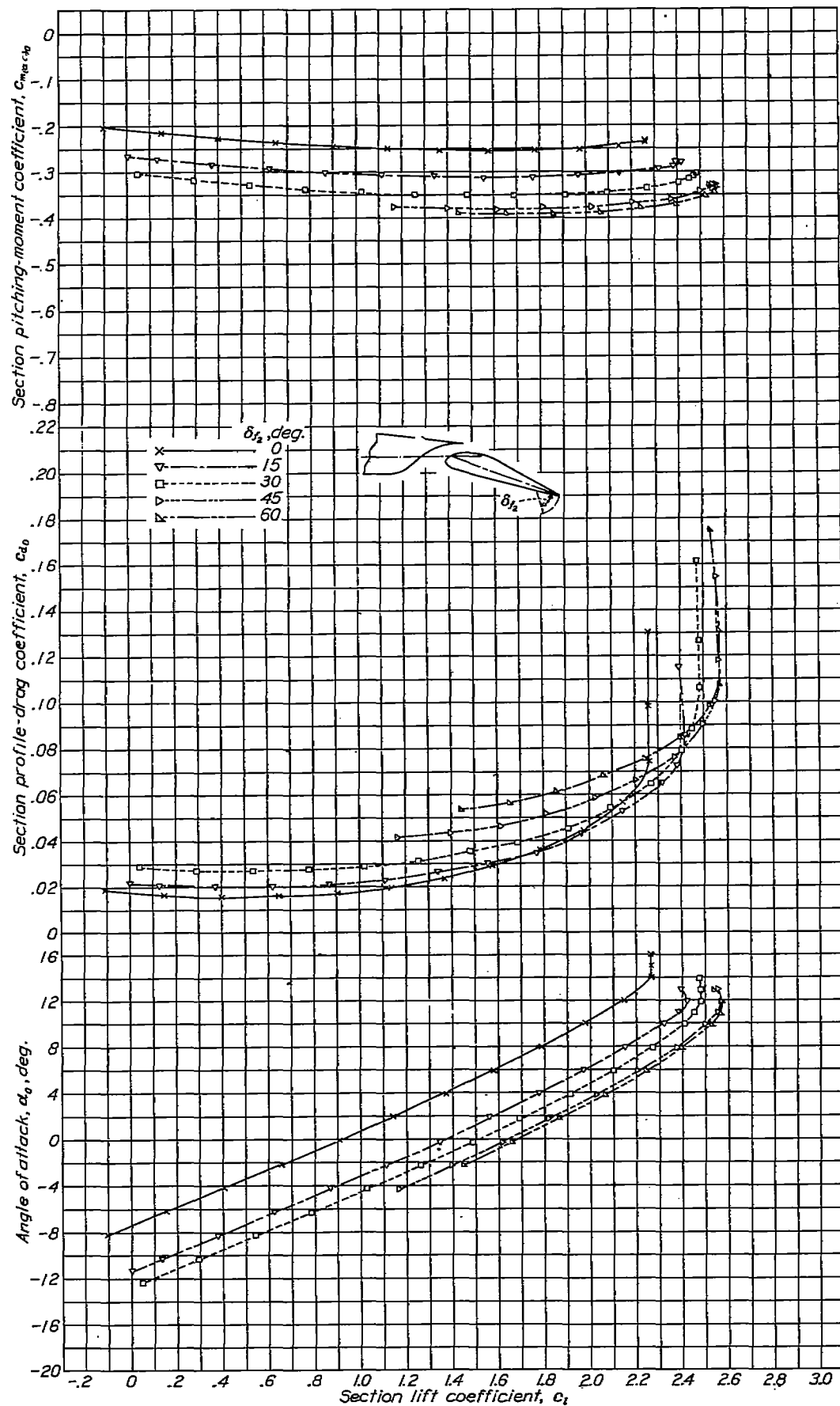
FIGURE 6.—Section characteristics of the N. A. G. A. 23012 airfoil with the main slotted flap deflected 20^\circ and the auxiliary 0.05c_w split flap deflected various amounts.
