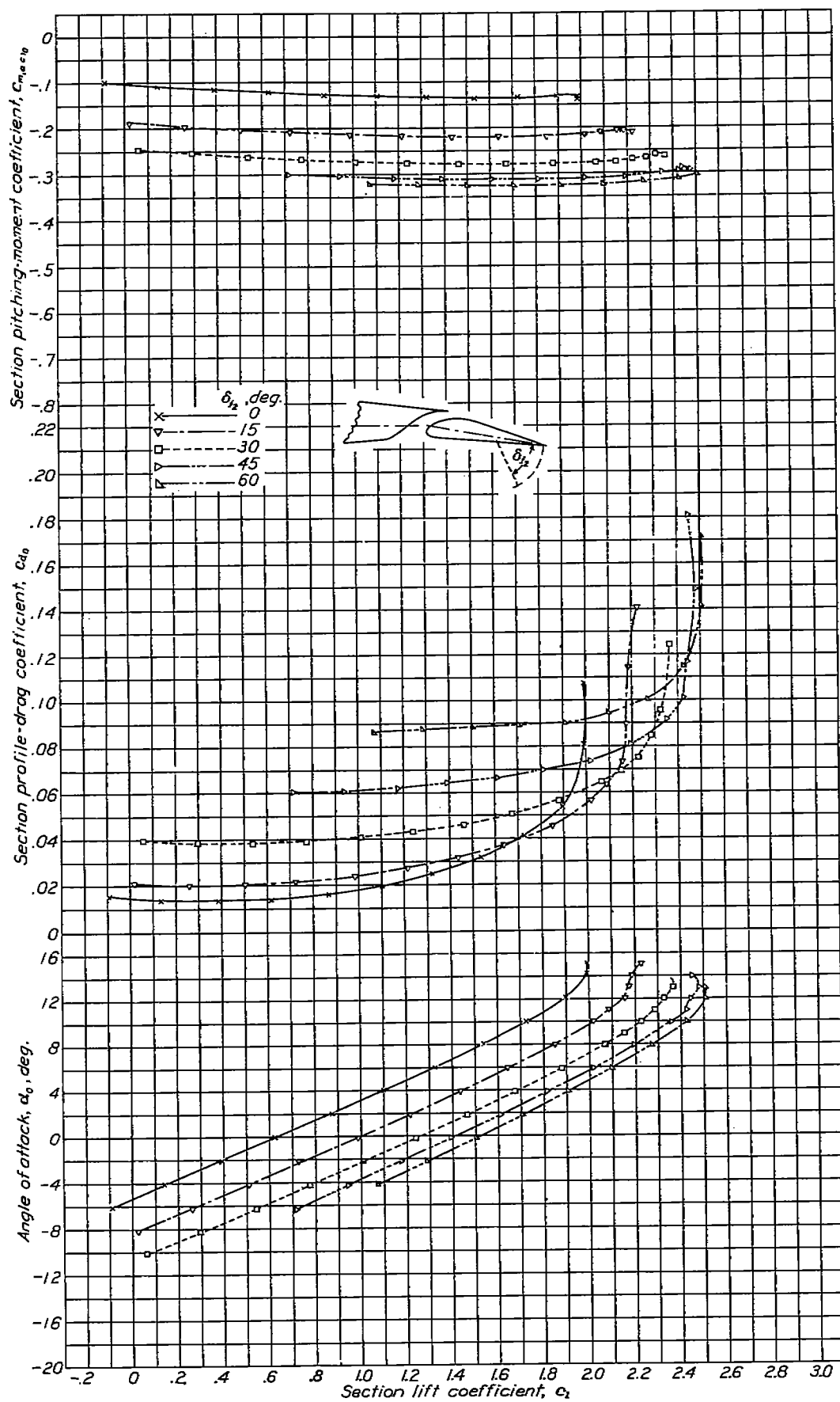
FIGURE 10.—Section characteristics of the N. A. C. A. 23012 airfoil with the main slotted flap deflected 10^\circ and the auxiliary 0.10c_s split flap deflected various amounts.
