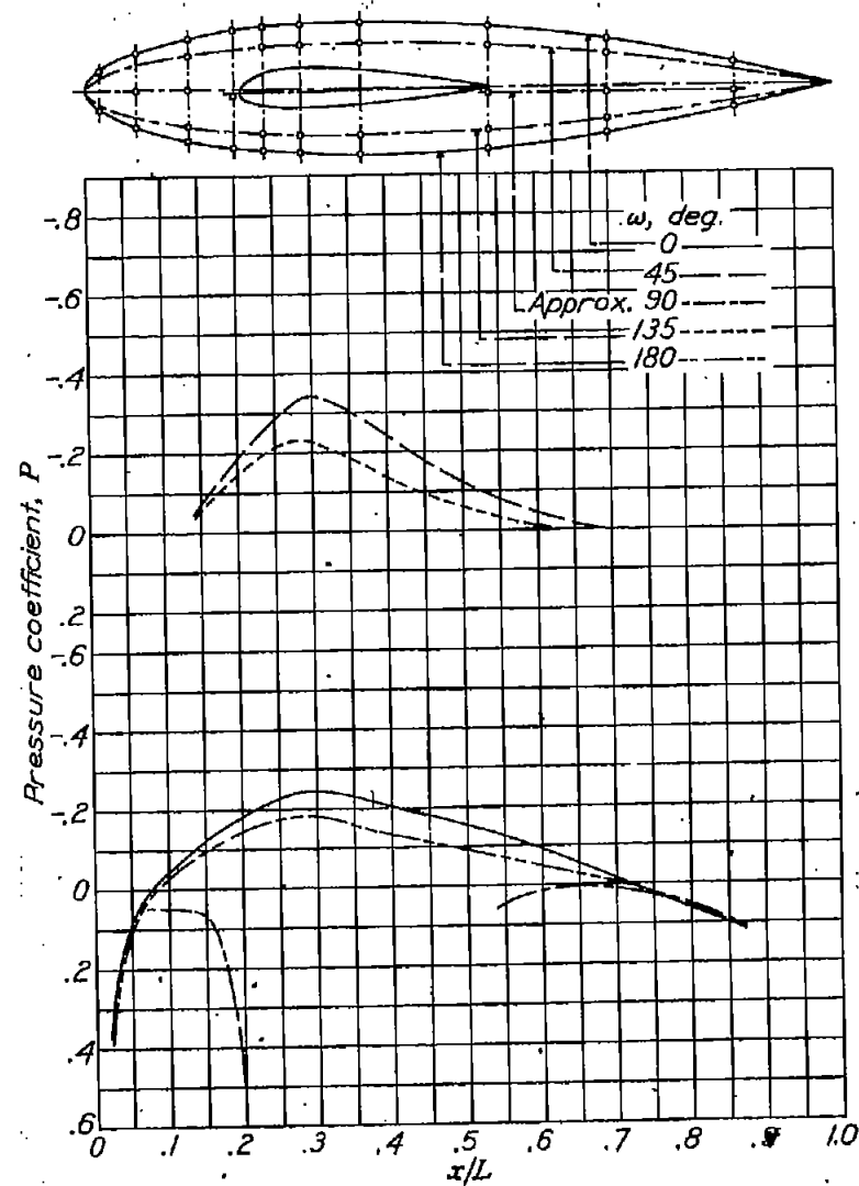
Figure 5.- Pressure distribution on fuselage. \alpha_p, 0^\circ ; M, 0.182 .
