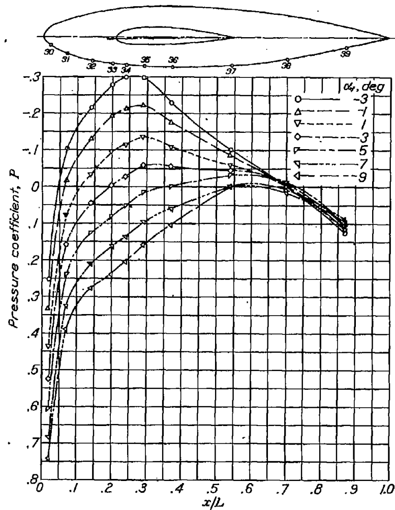
Figure 11.- Pressure distribution on fuselage. \alpha , 180^\circ ; M , 0.182.
