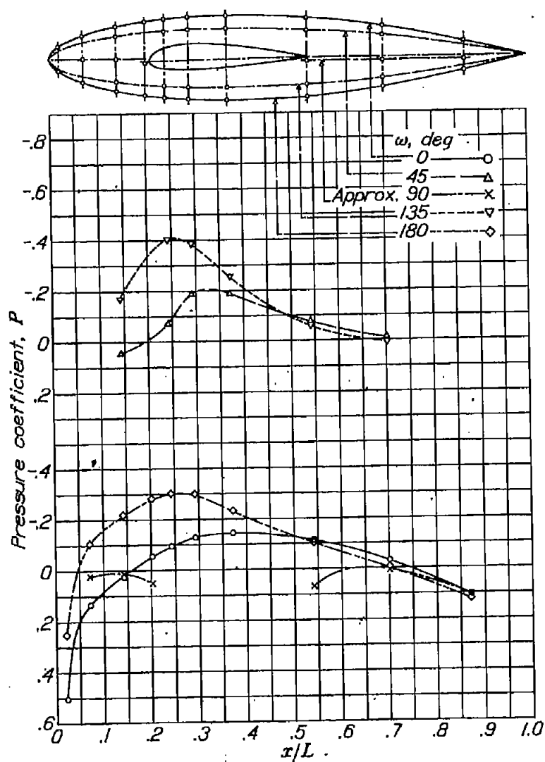
Figure 4.- Pressure distribution on fuselage. \alpha_p, -3^\circ ; M, 0.182 .
