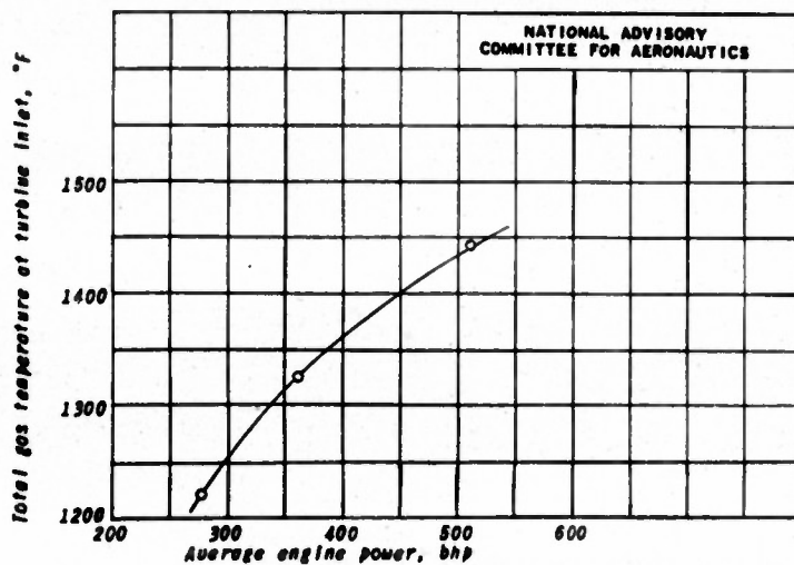
Figure 12. - Effect of engine power on exhaust-gas temperature of Pratt & Whitney R-1340-12. Engine speed, 2000 rpm; fuel-air ratio, 0.075.
