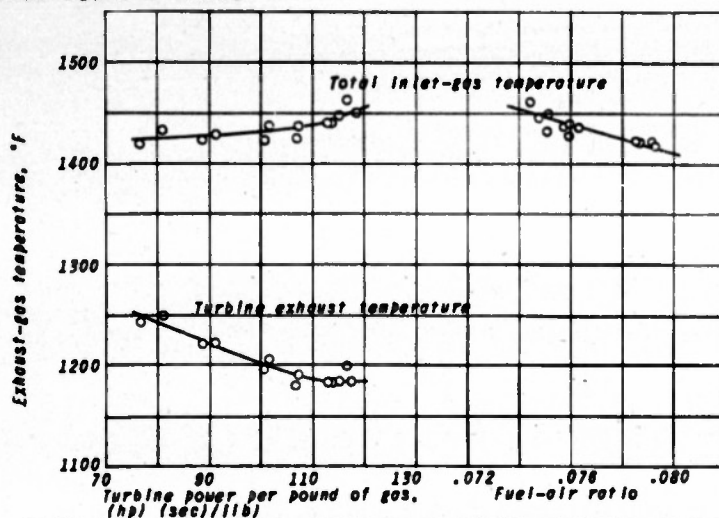
Figure 11. - Variation of exhaust-gas temperature of turbine outlet with turbine power. Average engine power, 513 horsepower; engine speed, 2000 rpm; exhaust pressure, 7.5 inches of mercury absolute.
