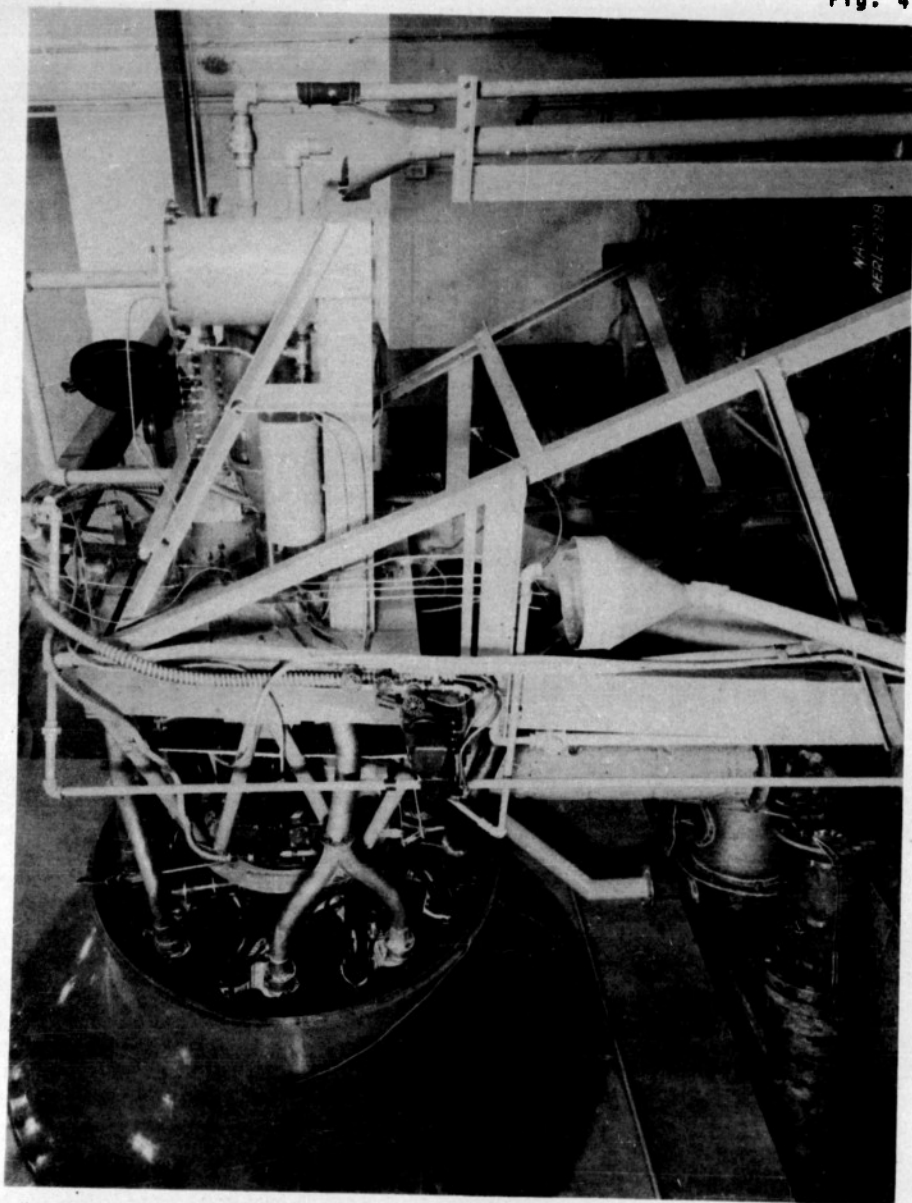
Figure 4. - Engine and blowdown turbine test setup.
