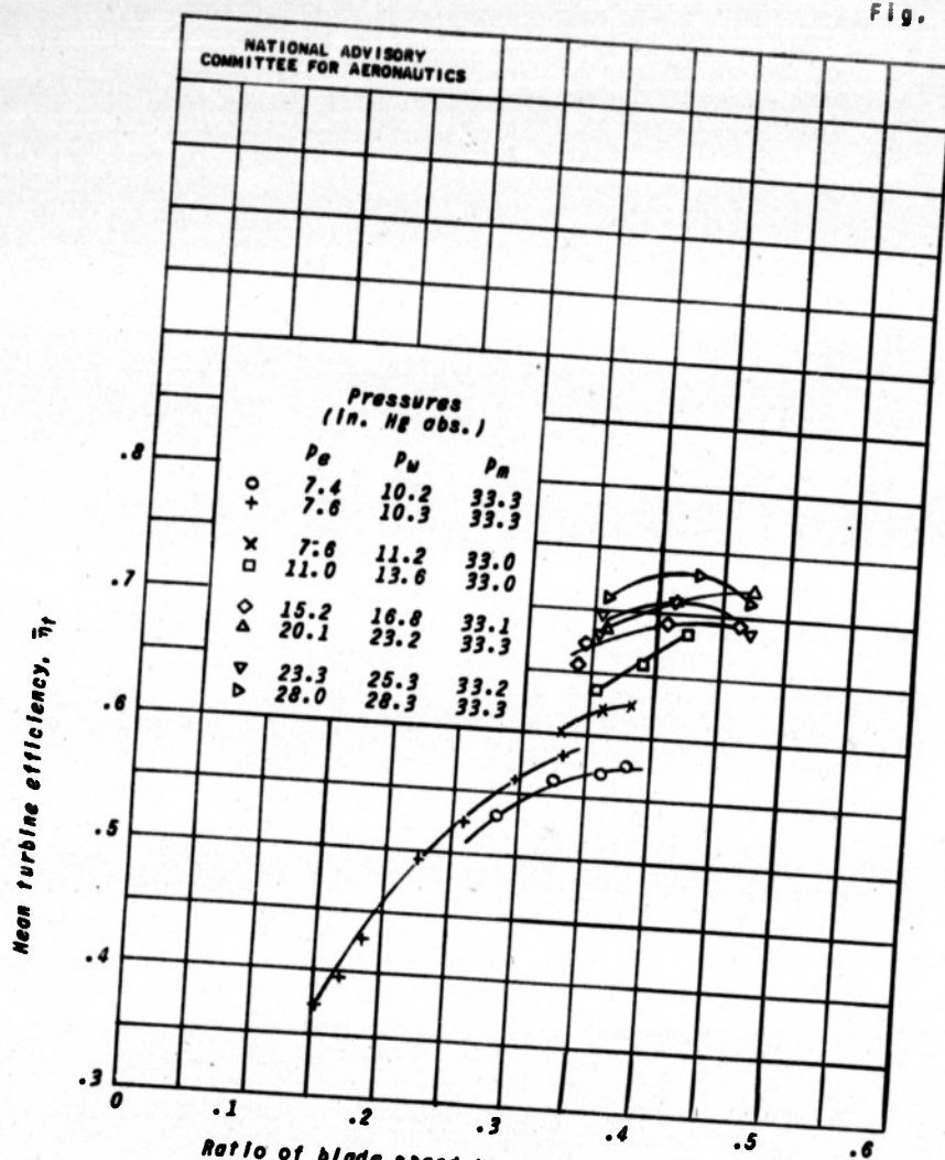
Figure 8. - Variation of mean turbine efficiency with ratio of blade speed to mean jet speed. Engine speed, 2000 rpm; full throttle.
