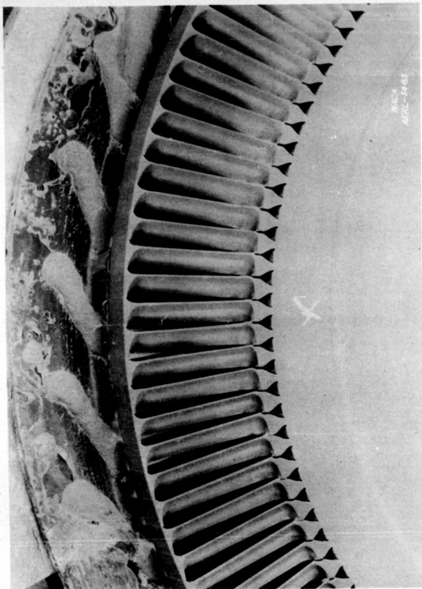
Figure 14. - Lead deposits on exit side of buckets.
