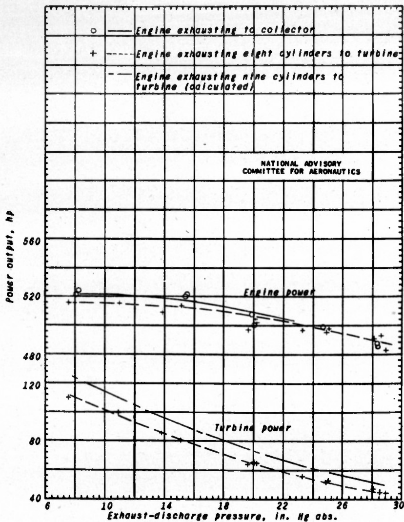
Figure 5. - Power output of Pratt & Whitney R-1340-12 engine and blowdown turbine. Engine speed, 2000 rpm. Data corrected to a carburetor-air temperature of 90° F and an inlet-manifold pressure of 33.5 inches of mercury absolute.
