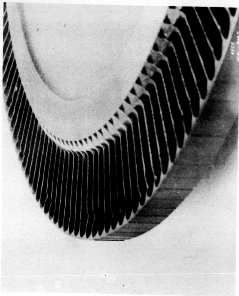
Figure 15. - Erosion and bending of leading edges of buckets.
