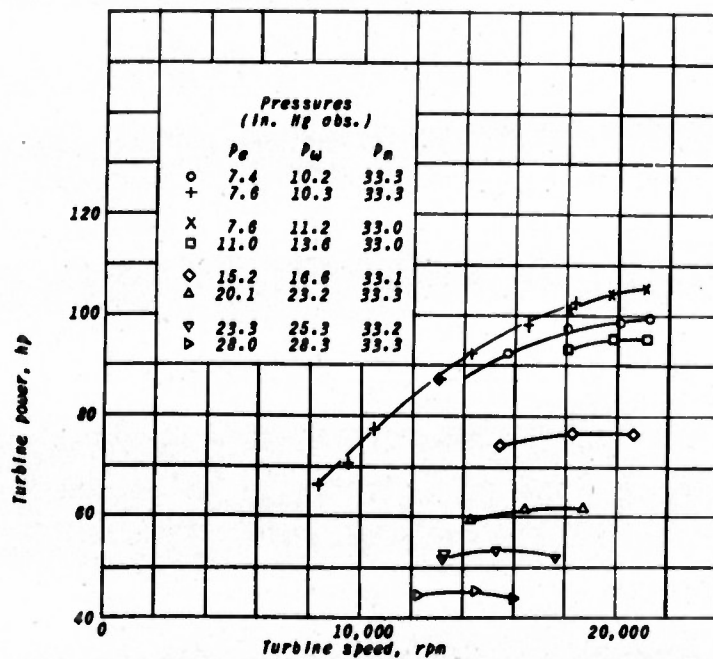
Figure 7. - Variation of turbine power with turbine speed. Engine speed, 2000 rpm; full throttle.
