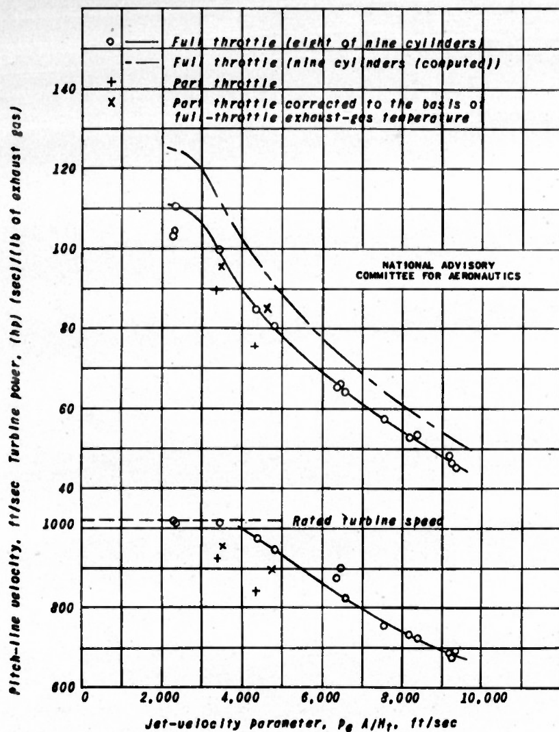
Figure 10. - Maximum turbine power output per pound of exhaust gas and optimum turbine speed. Engine speed, 2000 rpm.
