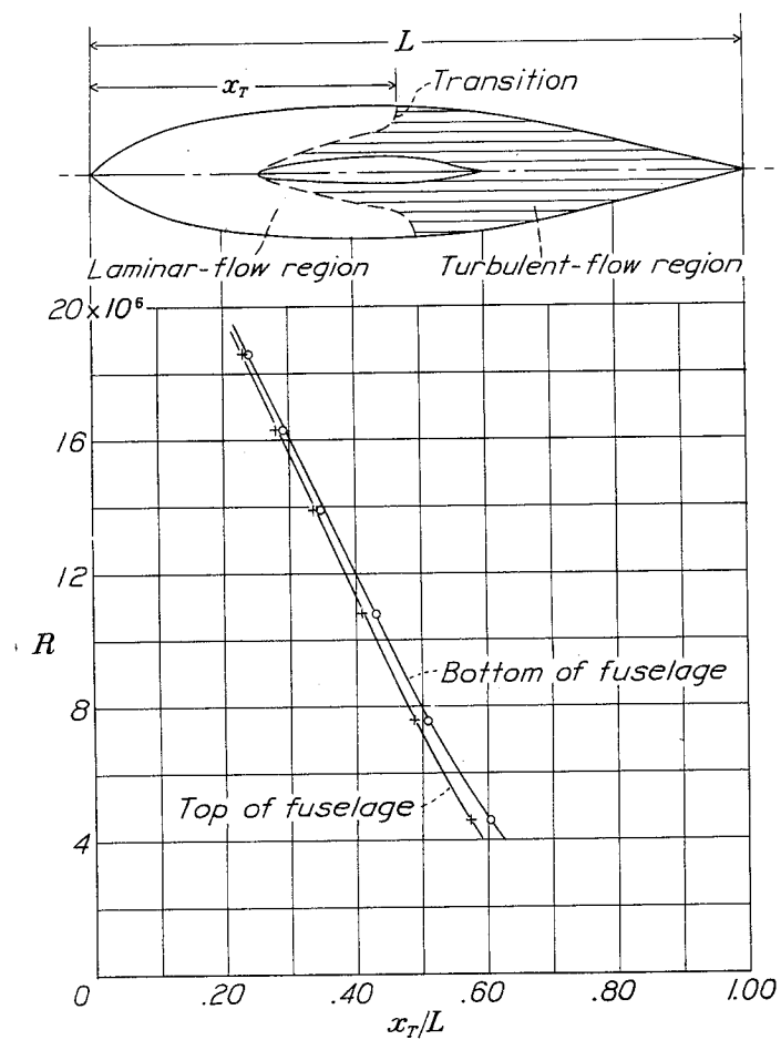
Figure 10.- Variation with Reynolds number of the location of the transition point on top and bottom of streamline body.
