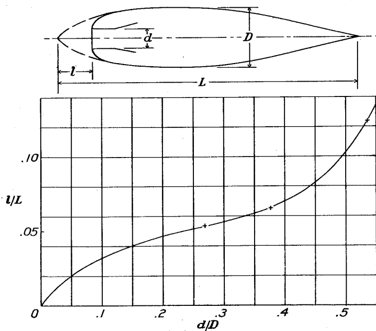
Figure 21.- Variation with duct diameter of the distance between the end of the nose and the tip of the streamline body.
