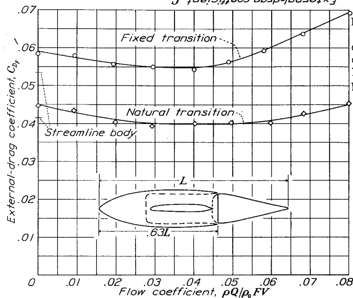
Figure 28a and b.- Variation with flow coefficient of the external-drag coefficients for nose inlet opening A combined with various tail outlet openings.
