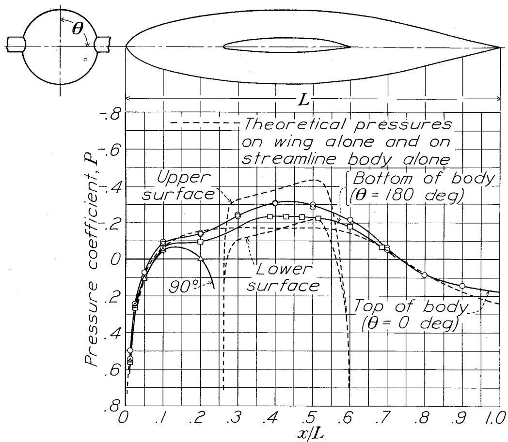
Figure 8.- Measured static-pressure distribution about streamline body mounted on NACA 27-212 airfoil compared with theoretical distribution on wing alone and body alone. M , 0.18; R , 7.6 \times 10^6 .
