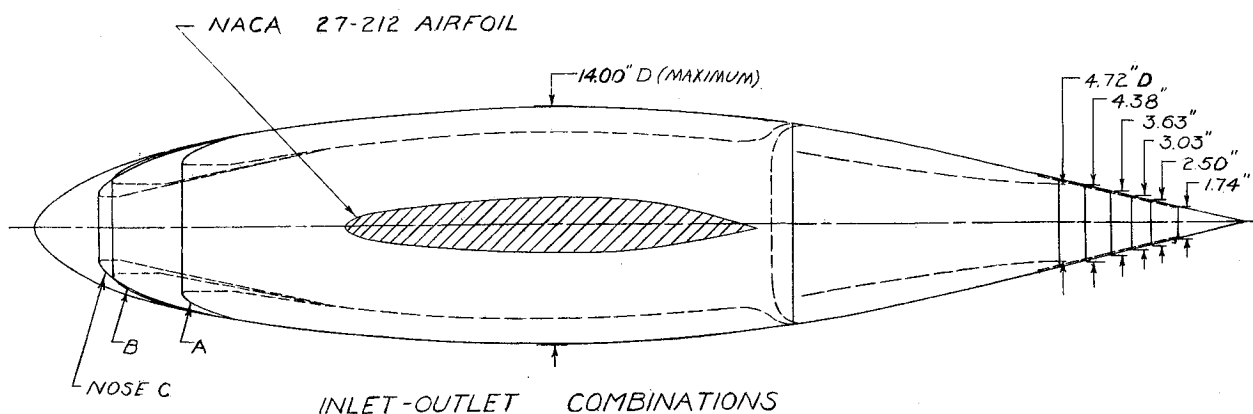
Figure 1.- Streamline body with general arrangement of inlet and outlet openings.
