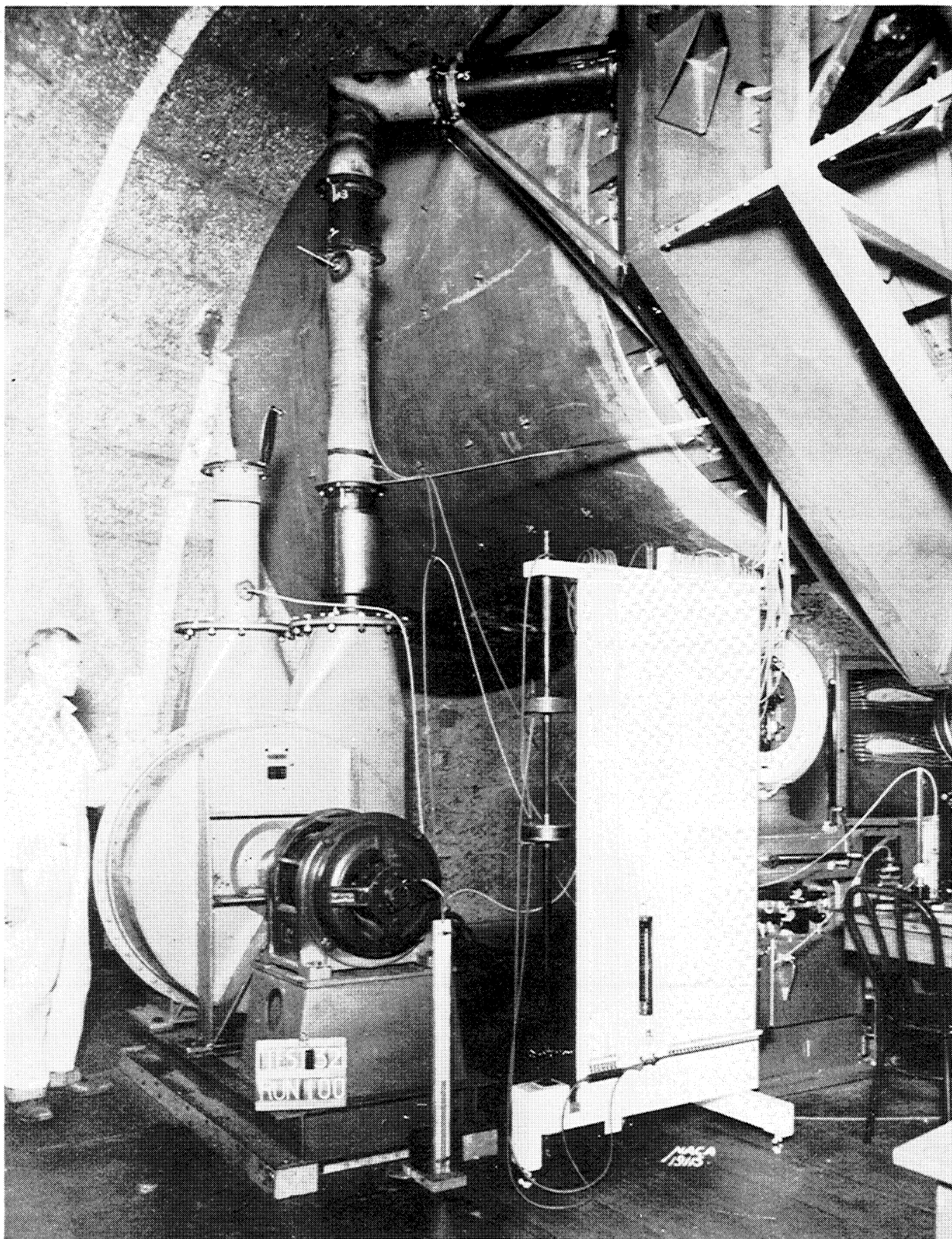
Figure 7. - General view of blower set-up in the test chamber of the 8-foot high-speed wind tunnel.
