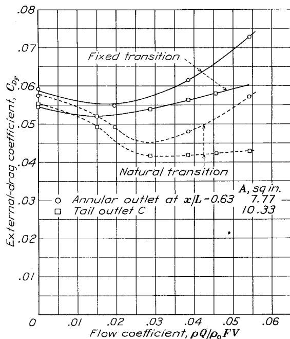
Figure 33.- Comparison of the external-drag coefficients of tail outlet C and the annular outlet at the 63-percent station of the fuselage. Nose B.
