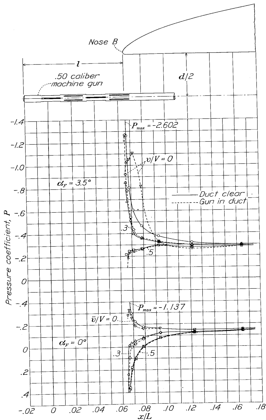
Figure 35.- The effect of the presence of a .50-caliber machine gun model in the inlet opening on static-pressure distribution on top of the body. Nose B, natural transition.
