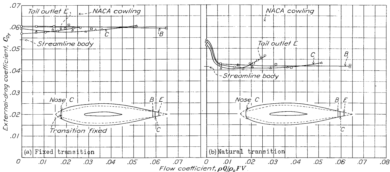
Figure 31a and b.- Variation with flow coefficient of the external-drag coefficients for nose inlet opening C combined with various tail outlet openings.
