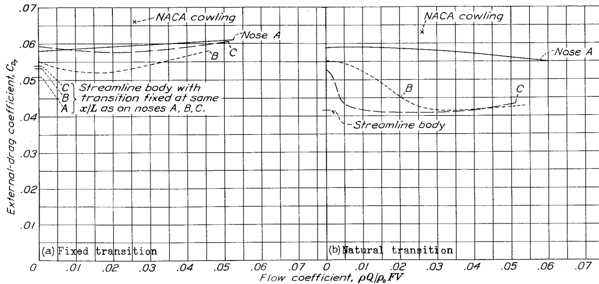
Figure 32.- Comparison of the external-drag coefficients of the three nose inlet openings tested with tail outlet opening C.
