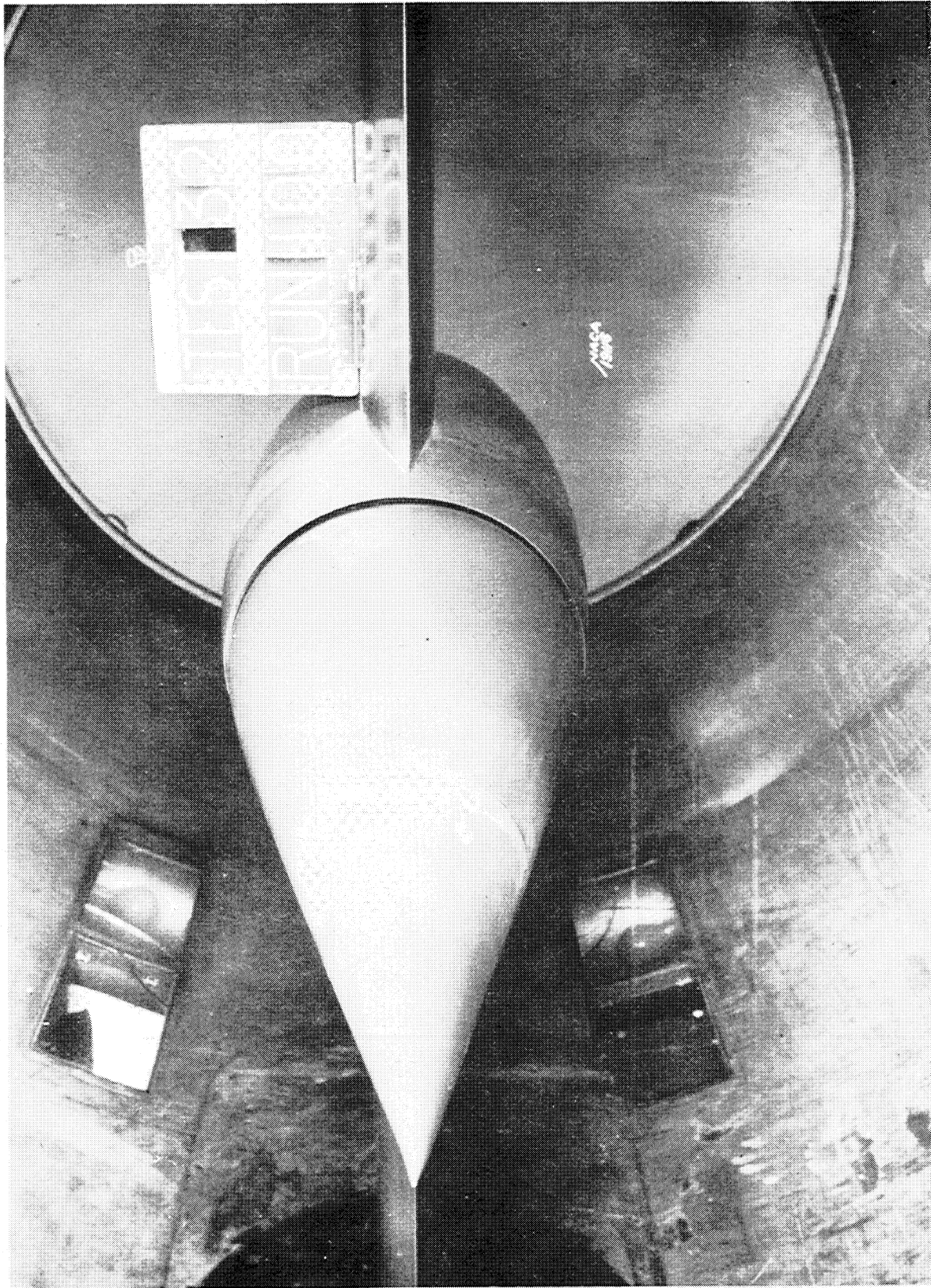
Figure 5.- Radial outlet opening at x = 0.63L .
