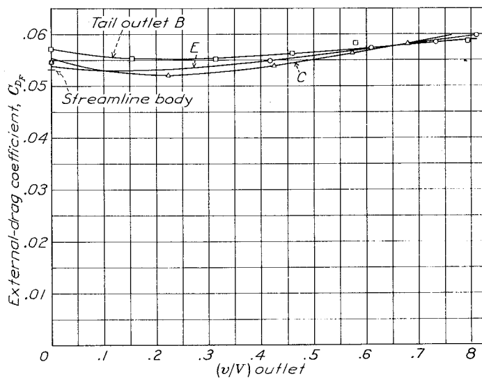
Figure 31a and b.- Variation with flow coefficient of the external-drag coefficients for nose inlet opening C combined with various tail outlet openings.
