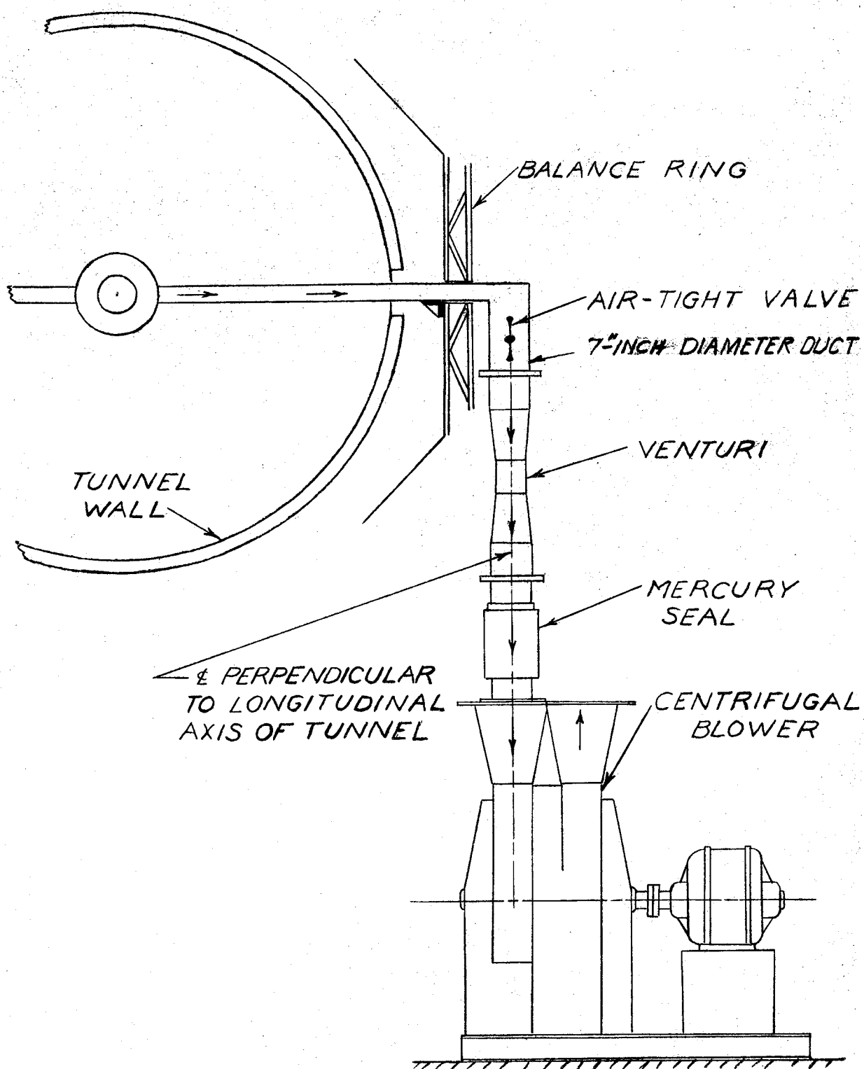
Figure 6.- Schematic diagram of set-up for tests with blower.
