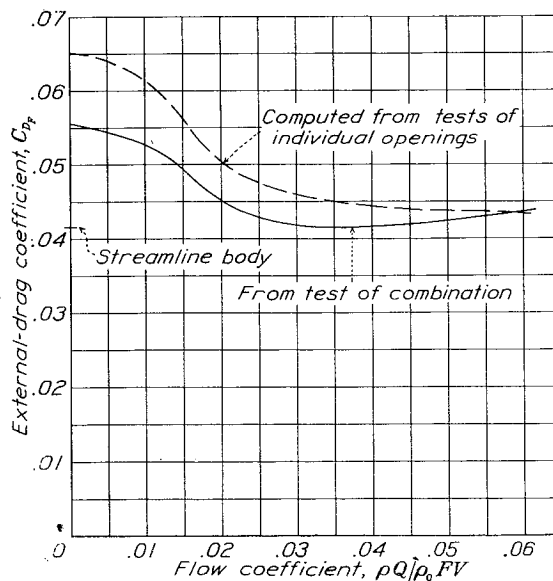
Figure 34.- The external-drag coefficient of the nose B - tail C combination compared with an estimate based on the drag increments obtained in the tests of the individual openings. Natural transition.
