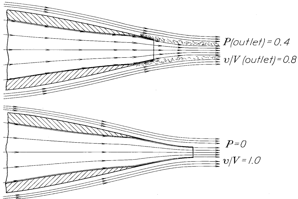
Figure 26.- Sketch of flow conditions (no internal losses) for a tail outlet opening similar to those tested and for a suggested improved type.
