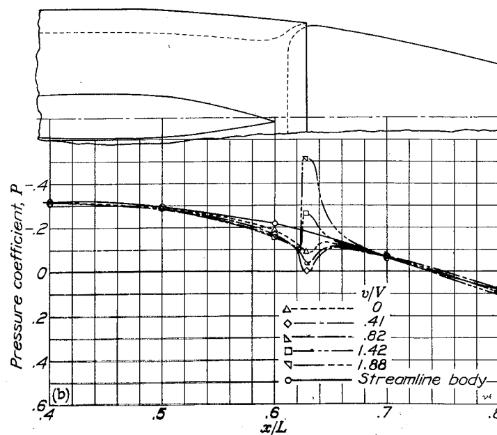
Figure 24b.- Opening at 63-percent station.
