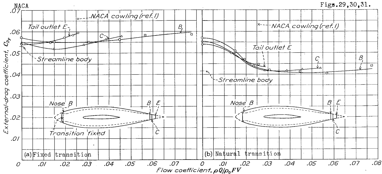
Figure 29a and b.- Variation with flow coefficient of the external-drag coefficients for nose inlet opening B combined with various tail outlet openings.
