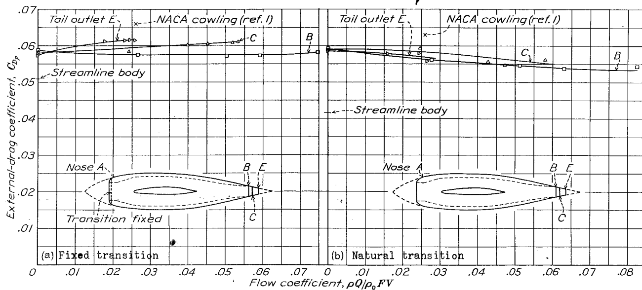
Figure 28a and b.- Variation with flow coefficient of the external-drag coefficients for nose inlet opening A combined with various tail outlet openings.
