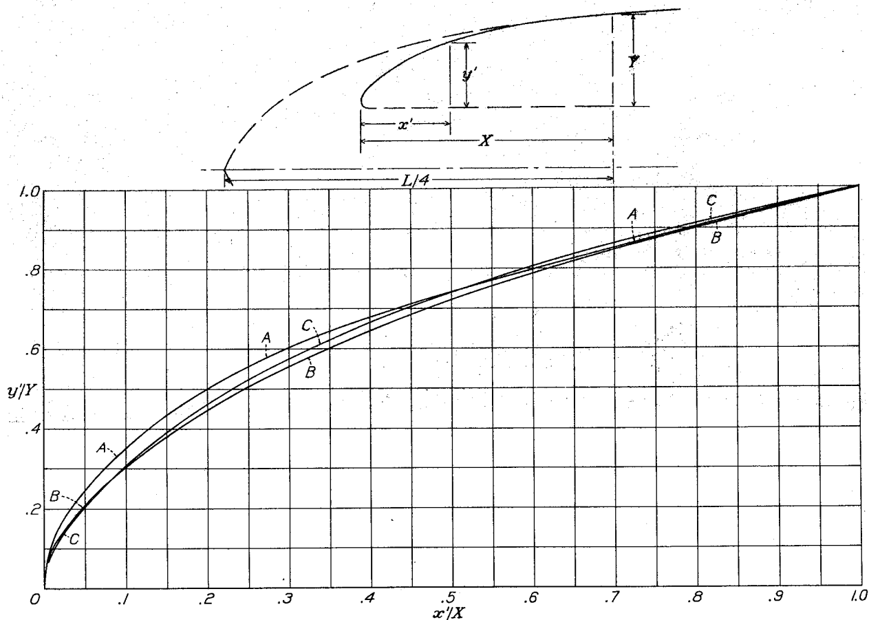
Figure 20.- Comparison of the three inlet opening nose profiles reduced to the same length and depth.
