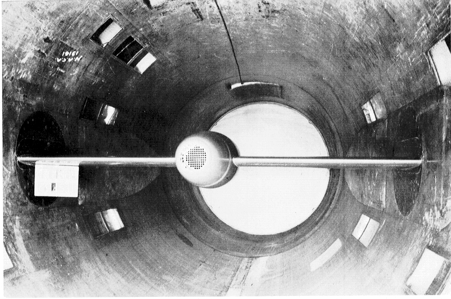
Figure 2. - Model installed in 8-foot high-speed wind tunnel. Nose B.
