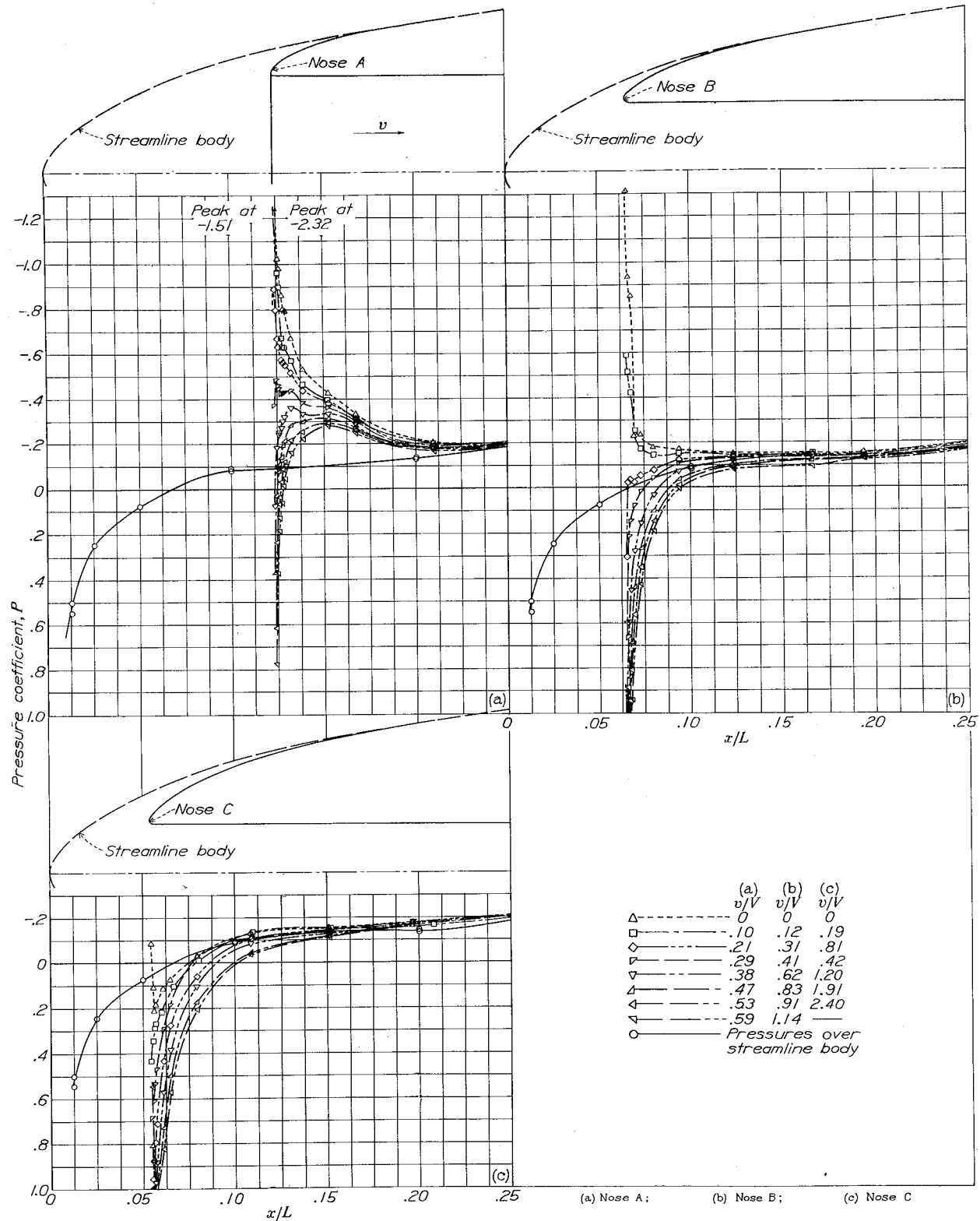
Figure 12.- The static pressure distribution over the nose inlet openings.
