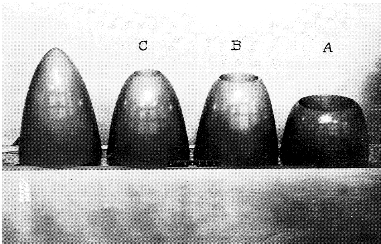
Figure 3. - Nose inlet openings compared with streamline nose.
