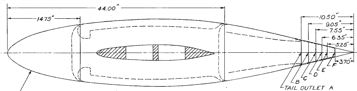
STREAMLINE BODY
