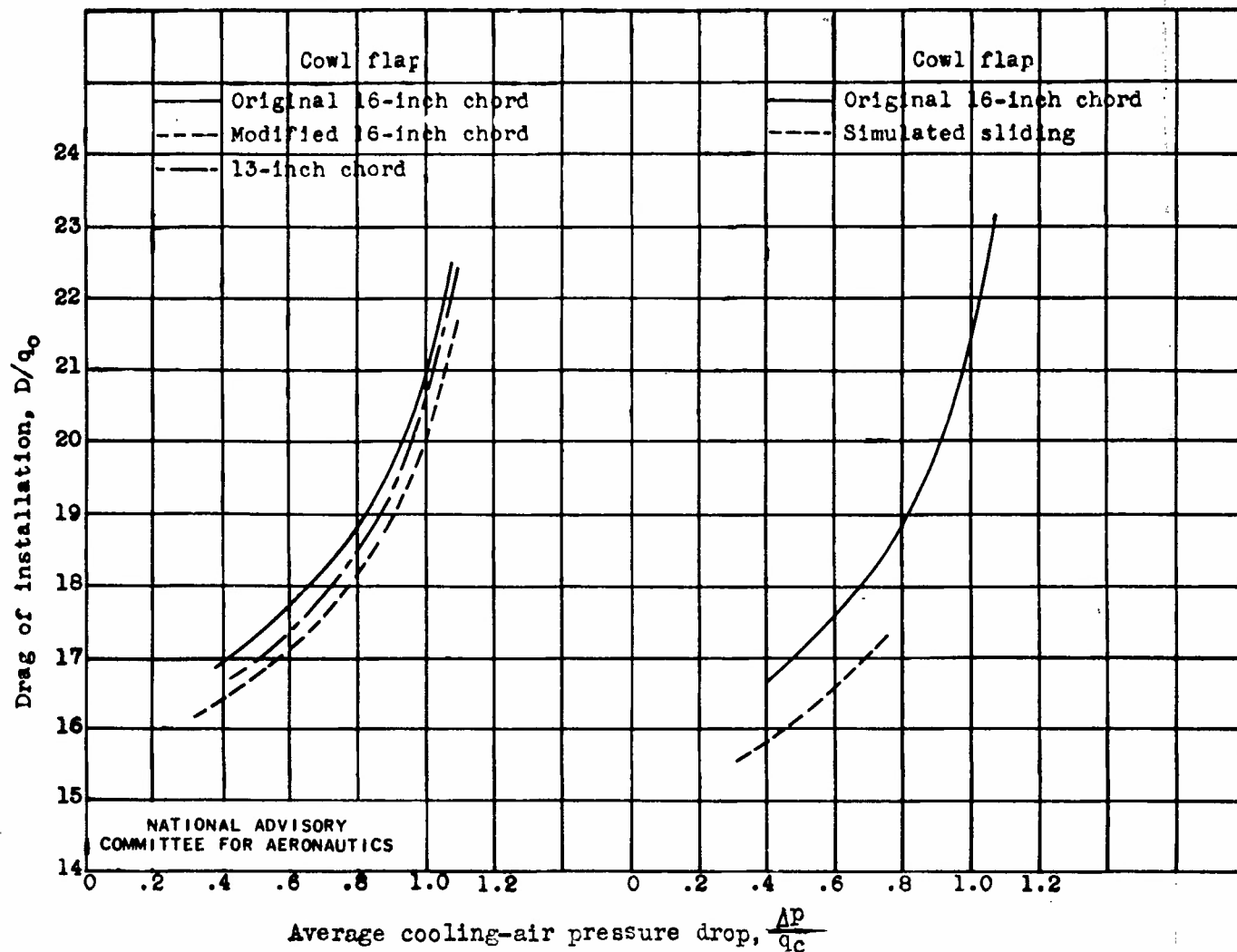
Figure 22. - Variation in drag of installation with average cooling-air pressure drop. Propeller removed; pressure altitude, 15,000 feet; indicated airspeed, 190 miles per hour.
