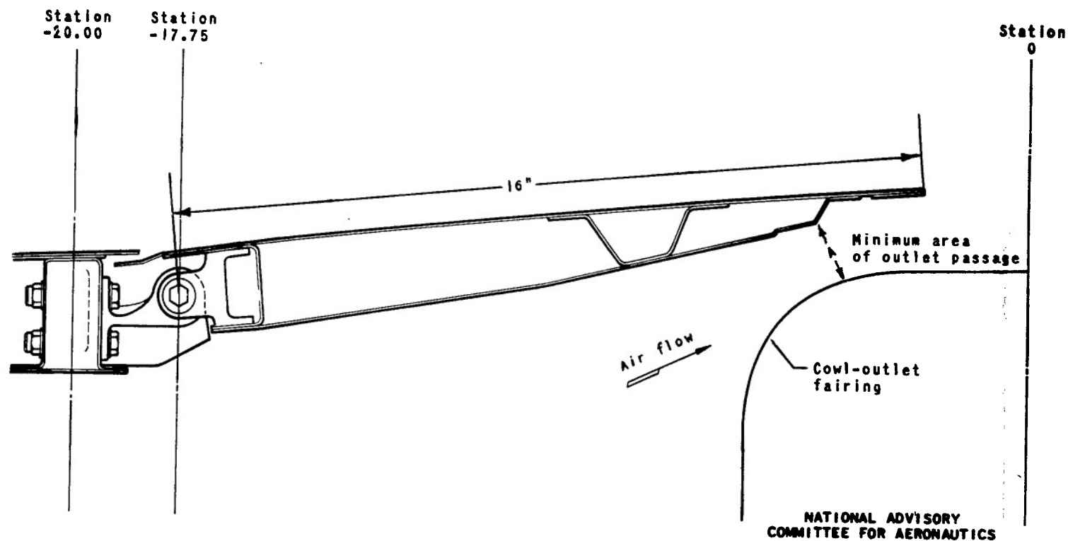
Figure 4. - Installation of original 16-inch-chord flap.
