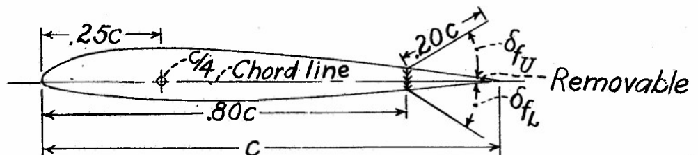
Typical section
