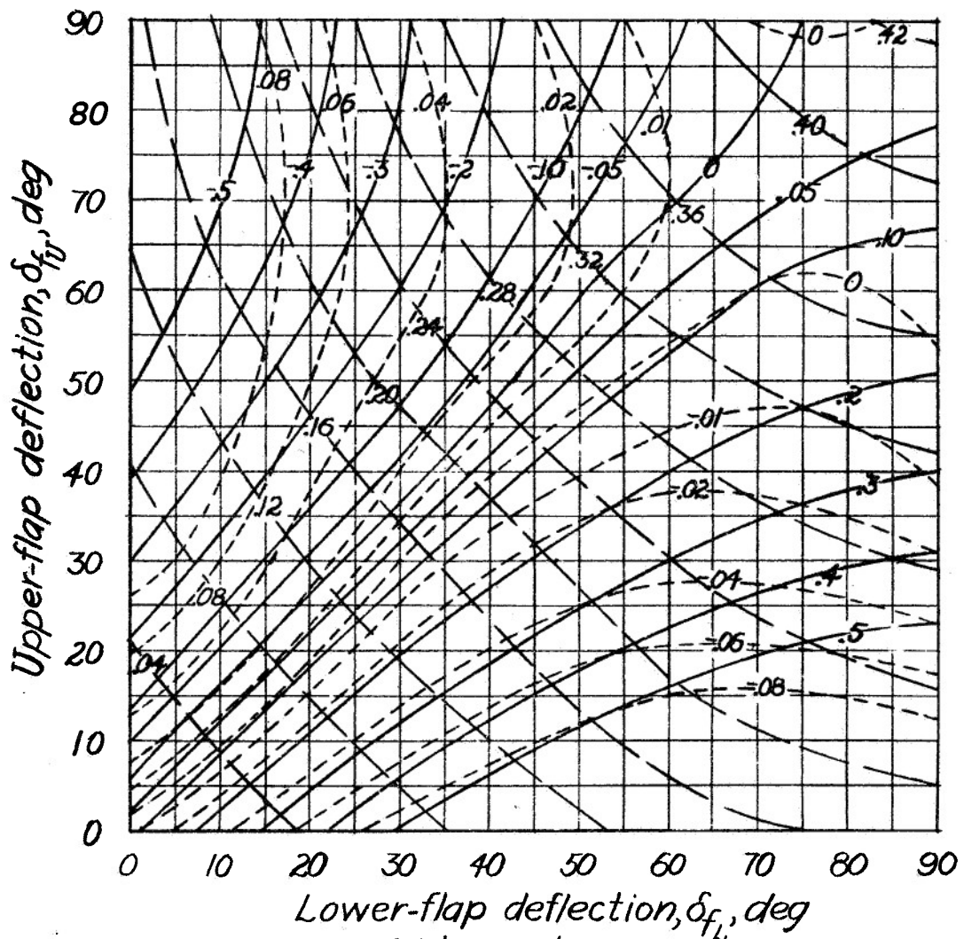
Figure 26.-Contours of C_L , C_D , and C_{m_{c/4}} at \alpha=0^\circ for the rectangular NACA 23012 airfoil with perforated double split flaps. Circular perforations remove 33.1 percent of original flap area.
