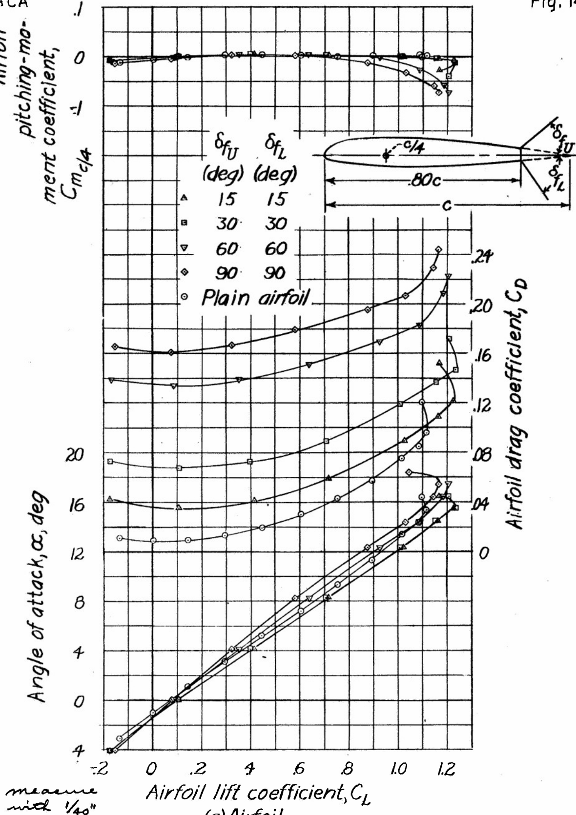
Figure 14 - Characteristics of the rectangular NACA 23012 airfoil with 0.20c by 0.40b perforated double split flaps. Circular perforations remove 33.1 percent of original flap area. Flap loads on segment 2. Equal upper and lower flap deflection.
