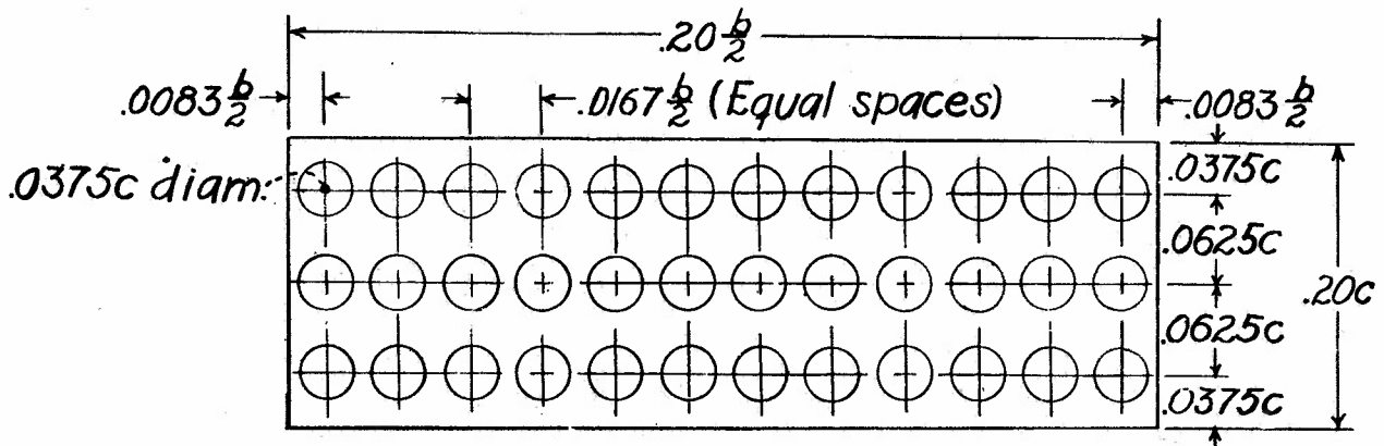
Flap detail
