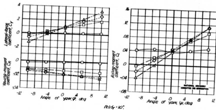
Figure 9 - Rolling-moment, yawing-moment, and lateral-force characteristics of tail B with various dihedral angles. \delta_e = \alpha = 0^\circ .
