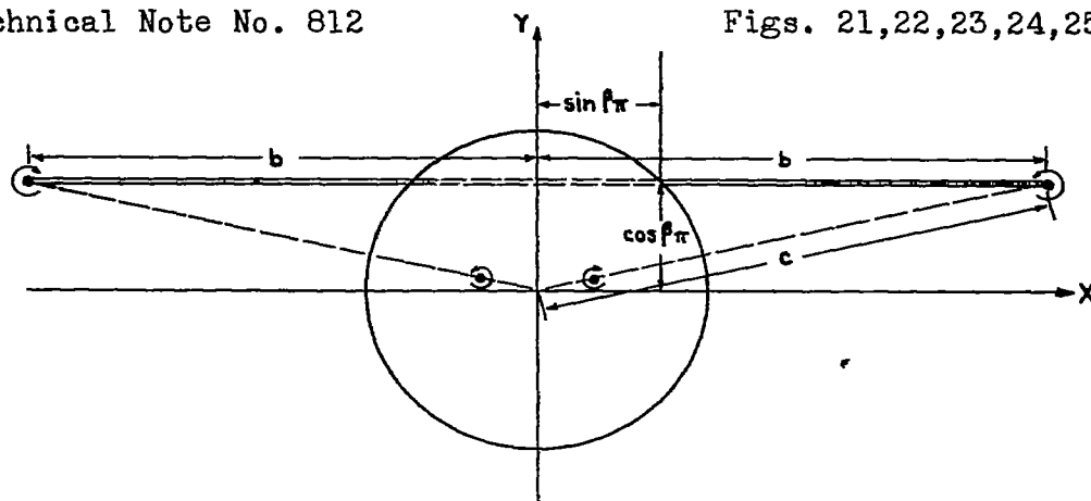
FIG. 21. - VORTEX SYSTEM OF HIGH-WING ENSEMBLE WITH CONSTANT CIRCULATION
