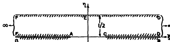
FIG. 9. - BOUNDING CONTOUR IN z -PLANE.
