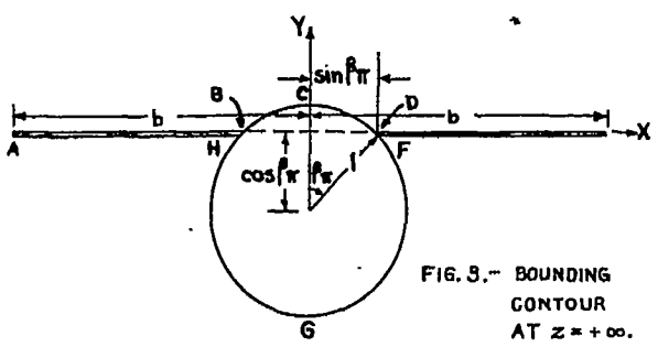
FIG. 3 BOUNDING CONTOUR AT Z = +\infty .
