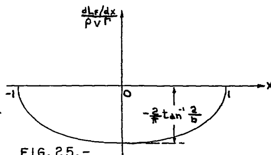
FIG. 25. - LIFT DISTRIBUTION OVER FUSELAGE OF EXTREME HIGH-WING ENSEMBLE.
