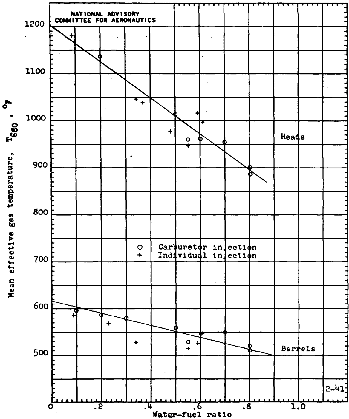
(a) Fuel-air ratio, 0.065.
