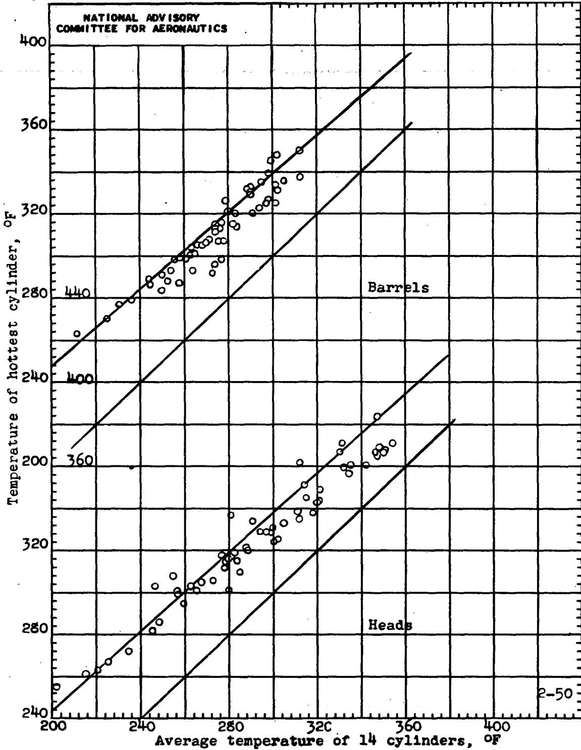
(b) Water injection through carburetor.
