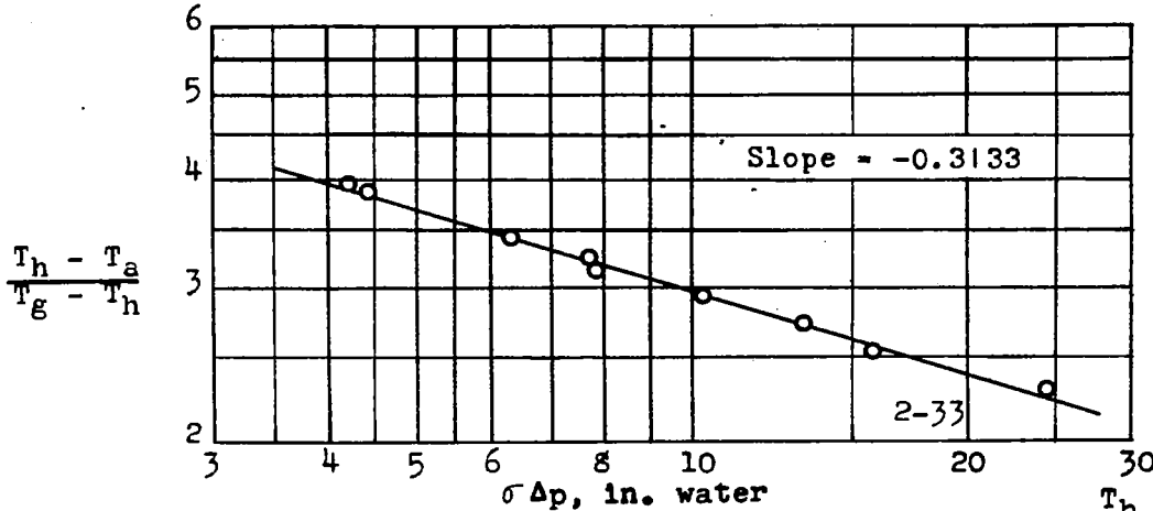
Figure 5. - Variation of cooling-temperature differential \frac{T_h - T_a}{T_g - T_h} with sea-level cooling-air pressure drop for cylinder heads.
