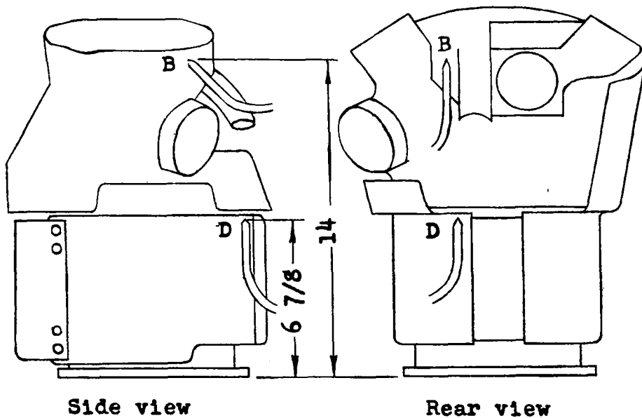
Rear-row cylinder
