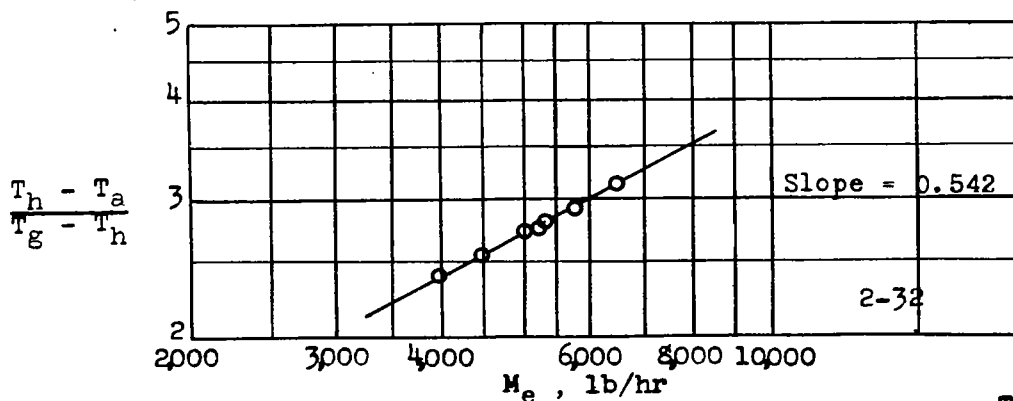
Figure 6. - Variation of cooling-temperature differential \frac{T_h - T_a}{T_g - T_h} with charge-air flow for cylinder heads. \sigma \Delta p , 13.7 inches water; fuel-air ratio, 0.08; Wright R-2600-8 engine.
