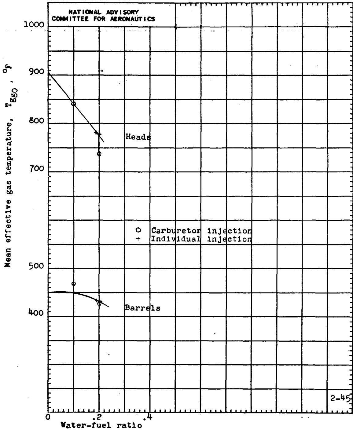
(e) Fuel-air ratio, 0.113.
