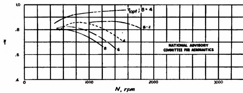
Figure 10.- Propeller efficiency. V = 150 miles per hour; P = 225 horsepower; \sigma_{0.7R} = 0.0345B .
