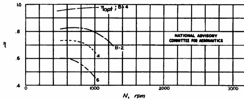
Figure 19.- Propeller efficiency. V = 200 miles per hour; P = 100 horsepower; \sigma_{0.7R} = 0.0345B .
