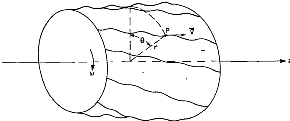
(a) Stream surface over four stages of multistage turbomachine.
