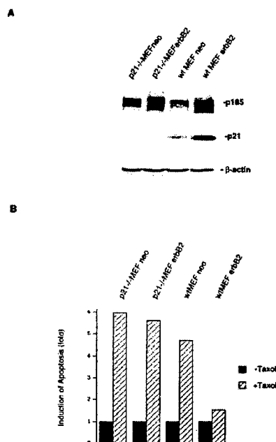
Figure 7. Overexpression of p185 ErbB2 Cannot Protect p21 -/- Mouse Embryonic Fibroblasts from Taxol-Induced Apoptosis
