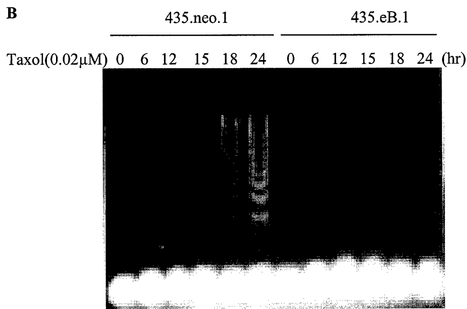
Figure 2. Taxol-induced Activation of p34 Cdc2 and Apoptosis are inhibited in p185-overexpressing 435.eB1 Cells.
