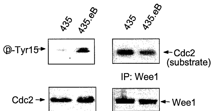
Figure 3. Increased phosphorylation on Cdc2-Tyr15 in p185 ErbB2 -overexpressing 435.eB transfectants.
