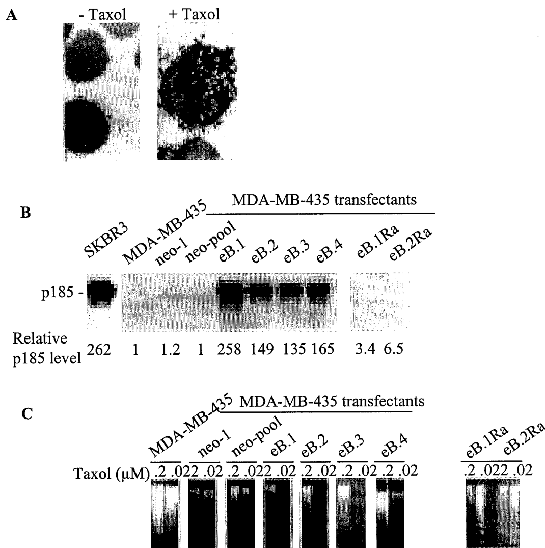
Figure 1. Overexpression of p185 ErbB2 inhibited Taxol-Mediated Apoptosis.
