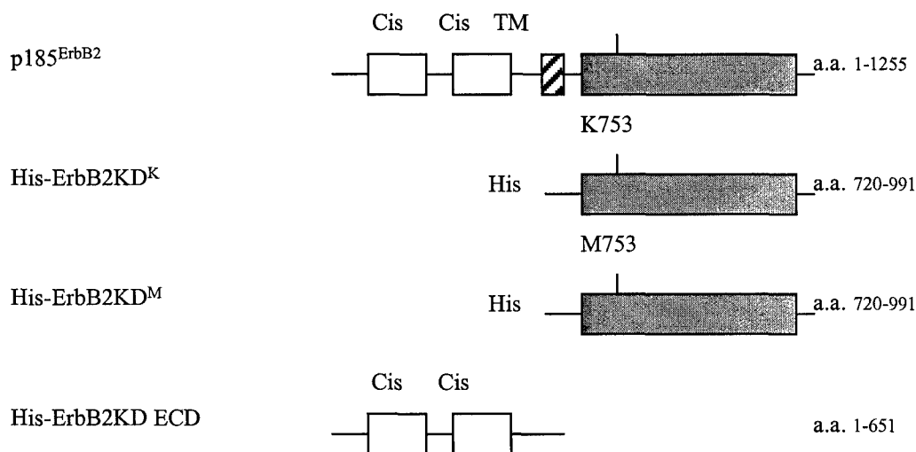
Figure 6. Diagram of the wild-type full-length p185 ErbB2 , His-tagged wild-type kinase domain of ErbB2 (His-ErbB2KDK K ), mutant kinase domain of ErbB2 (His-ErbB2KDM M ), and wild-type extracellular domain of ErbB2 (His-ErbB2KDECD). The amino acids (a. a.) relative to the wild-type full-length p185 ErbB2 included in each recombinant protein are indicated at right.
