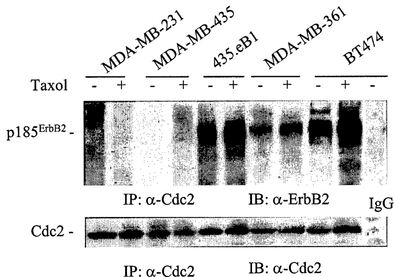
Figure 4. Association of p185 ErbB2 with p34 Cdc2 in vivo. The indicated cell lines were cultured in the absence (-) or presence (+) of Taxol (0.02 \mu M) for 24 hr. Total protein (500 \mu g) was immunoprecipitated for p34 Cdc2 . Immunocomplexes were resolved on 6-12% gradient SDS-PAGE, Cdc2-associated p185 ErbB2 and immunoprecipitated p34 Cdc2 were analyzed by immunoblotting for p185 ErbB2 or p34 Cdc2 .
