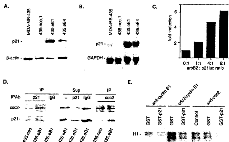
Figure 5. p185 ErbB2 Upregulates p21 Cip1 , which Inhibits p34 Cdc2
