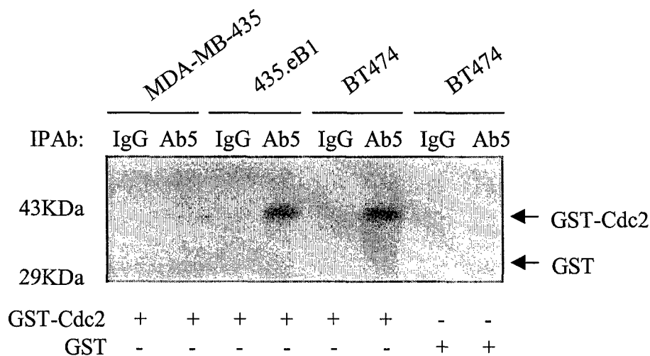
Figure 5. Phosphorylation of GST-Cdc2N50 by p185 ErbB2 complex. Protein lysates (1mg) from the indicated cell lines were immunoprecipitated using wither antibodies against the extracellular domain p185 ErbB2 (Ab5) or mouse IgG (control); immunocomplexes were subjected to kinase assays with [ 32 P]γ-ATP using either GST-Cdc2N50 or GST as substrates.
