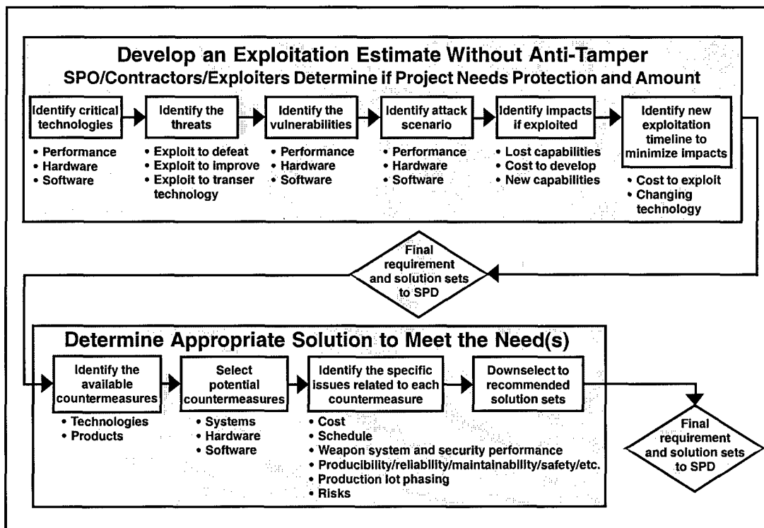
Figure 1. Determining Anti-Tamper Requirements
