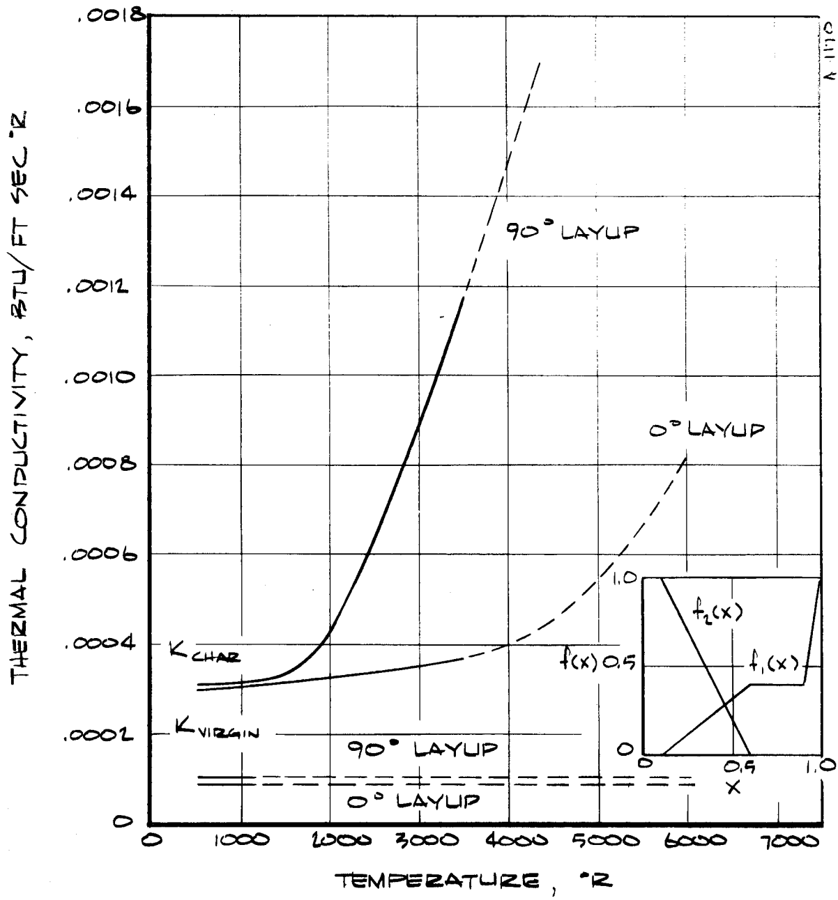
FIGURE 3-10 THERMAL CONDUCTIVITY FOR MXS-113 SILICA PHENOLIC
