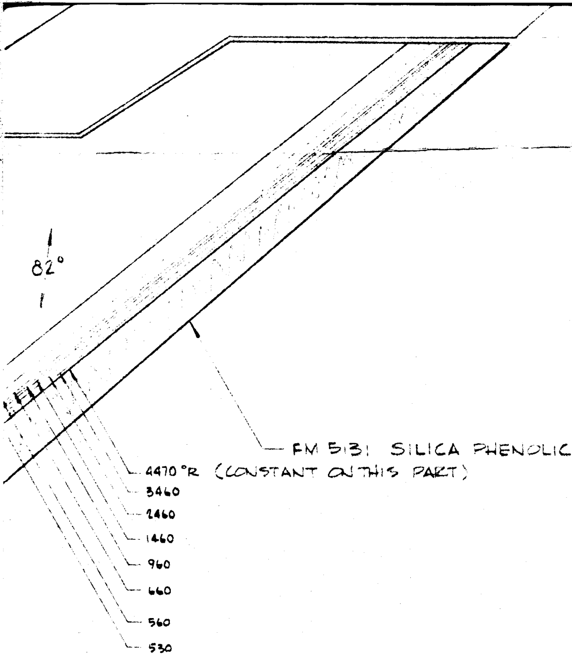
FIGURE 2-19 SURFACE RECESSION AND ISOTHERMS FOR THE NOSE OF THE 260-SL-3 NOZZLE AT THE END OF THE FIRING (RE POSITION)
