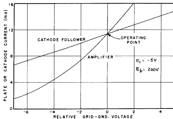
Figure 10 - Dynamic characteristics of 6C4 with 1000-ohm load
